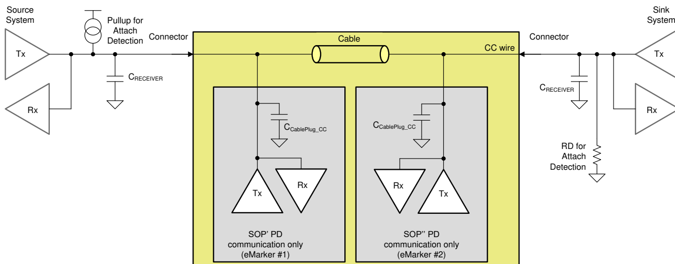
图 8-10. Example USB-PD Multi-Drop Configuration
