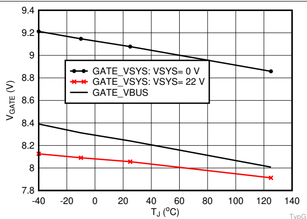
图 6-5. V_{GATE\_VBUS\_ON} vs. Temperature for TPS25730S
