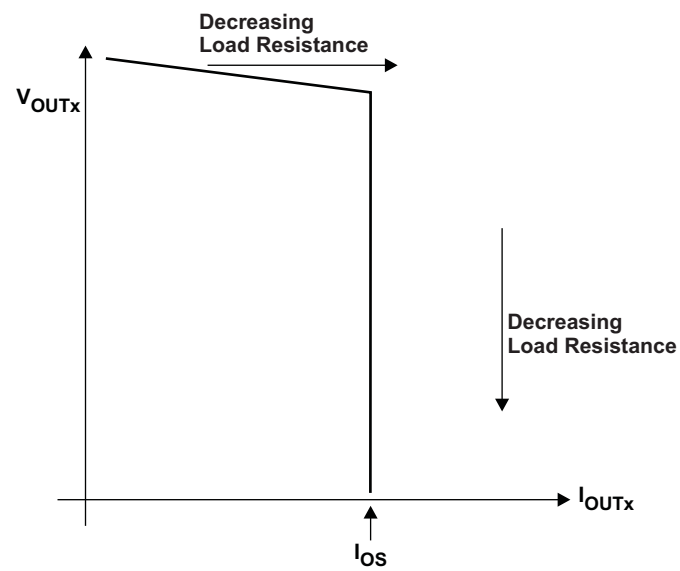
Figure 11. Output Voltage vs. Current-Limit Threshold
