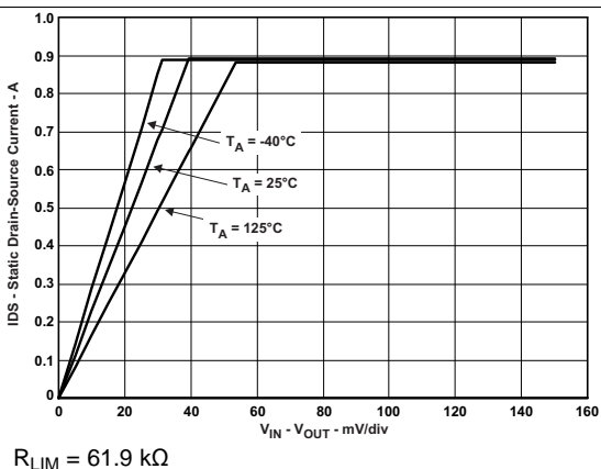
Figure 7. Switch Current Vs. Drain-Source Voltage Across Switch
