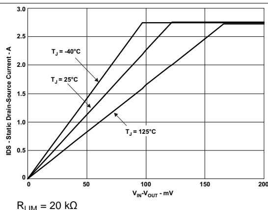
Figure 8. Switch Current vs. Drain-Source Voltage Across Switch
