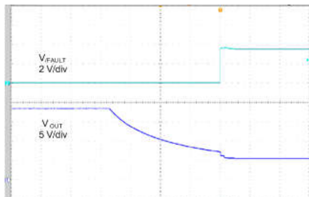
t = 100 ms/div 图 6-28. OUT Short-to-Battery Recovery
