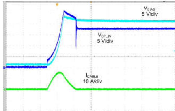
图 9-10. DC-DC Input Is Floating, DP_IN Shorted to Battery
