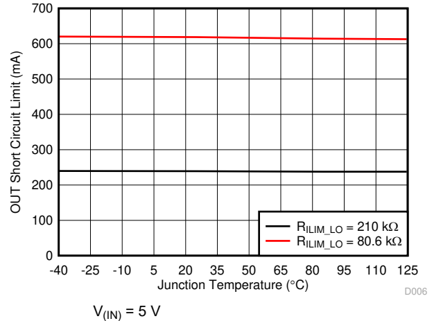
图 6-6. OUT Short-Circuit Current Limit vs Temperature II
