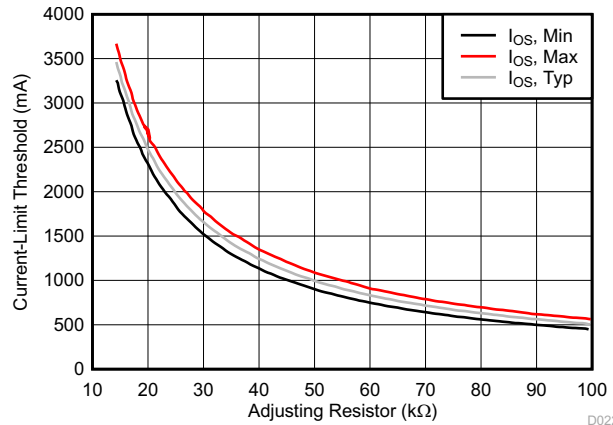
图 8-4. Current-Limit Setting vs Adjusting Resistor I
