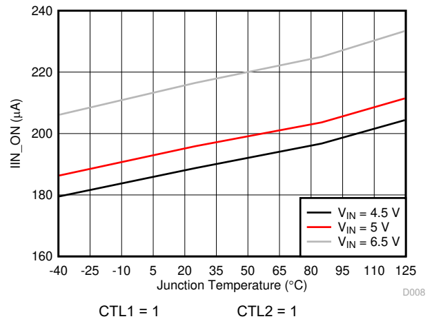
图 6-8. Enabled IN Supply Current - CDP (11) vs Temperature
