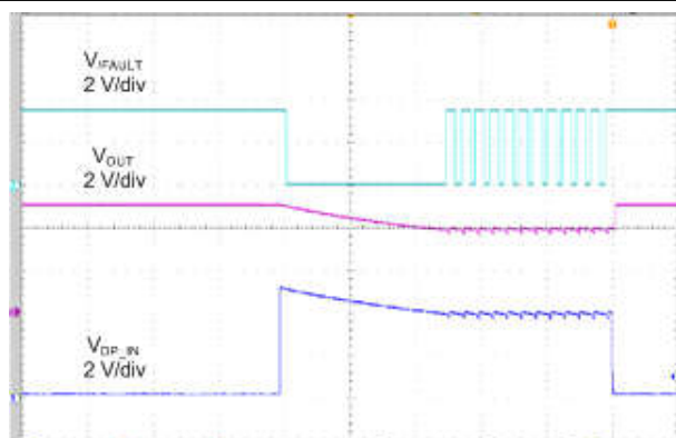
R_{BIAS} = 5.1\text{ k}\Omega t = 200 ms/div 图 6-32. DP_IN Short-to- V_{BUS} and Recovery
