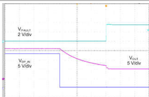
R_{BIAS} = 5.1\text{ k}\Omega t = 100 ms/div 图 6-30. DP_IN Short-to-Battery Recovery
