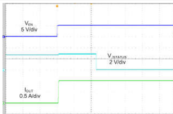
图 6-23. Short Circuit to No Load (CDP)
