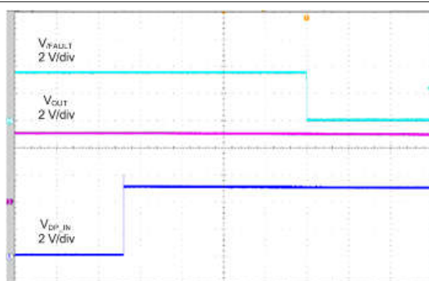
R_{BIAS} = 5.1\text{ k}\Omega t = 4 ms/div 图 6-31. DP_IN Short to V_{BUS}
