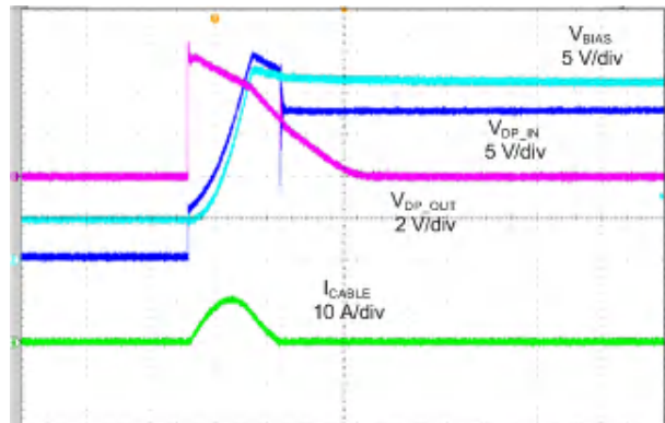
图 9-11. Enabled, DP_IN Shorted to Battery
