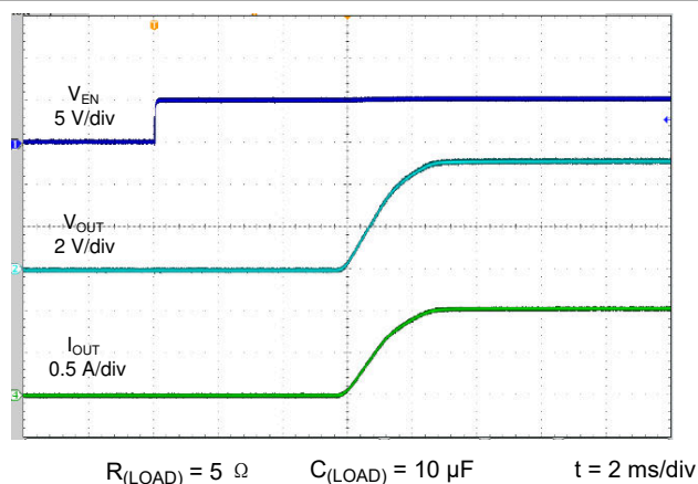
图 6-18. Turnon Response
