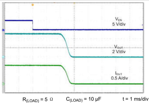
图 6-19. Turnoff Response
