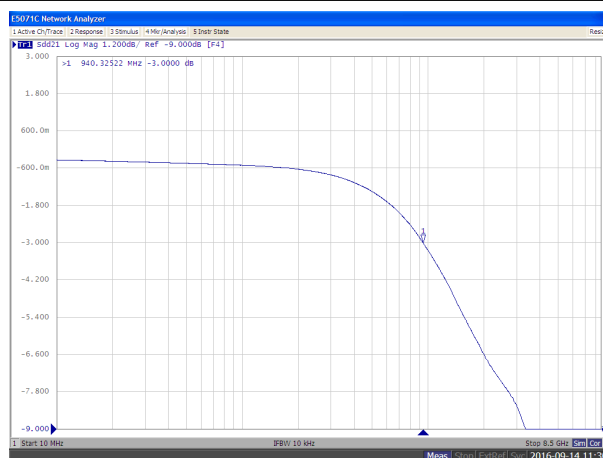
图 6-33. Data Transmission Characteristics vs Frequency
