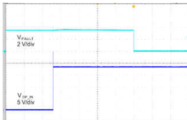
t = 4 ms/div 图 6-29. DP_IN Short to Battery
