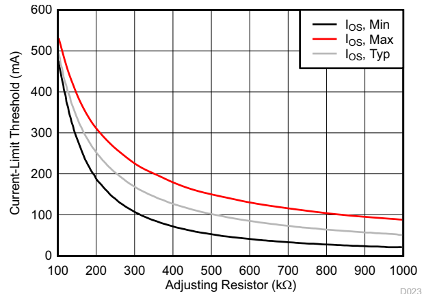
图 8-5. Current-Limit Setting vs Adjusting Resistor II
