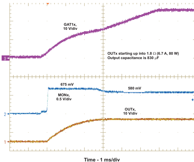
Figure 12. Startup into 80 Watt, 830 \mu\text{F} Load
