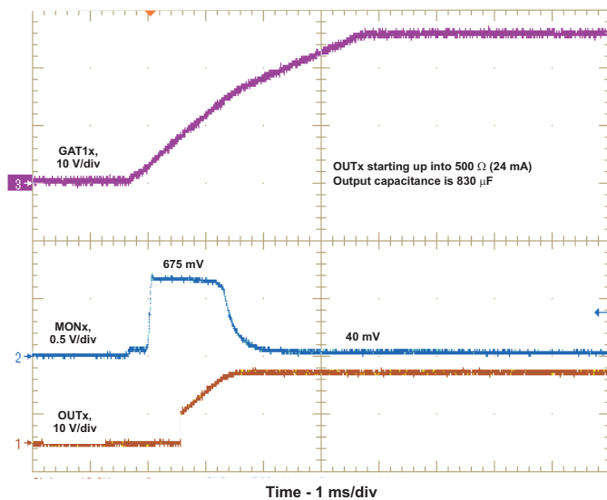
Figure 11. Startup into 500 \Omega , 830 \mu\text{F} Load
