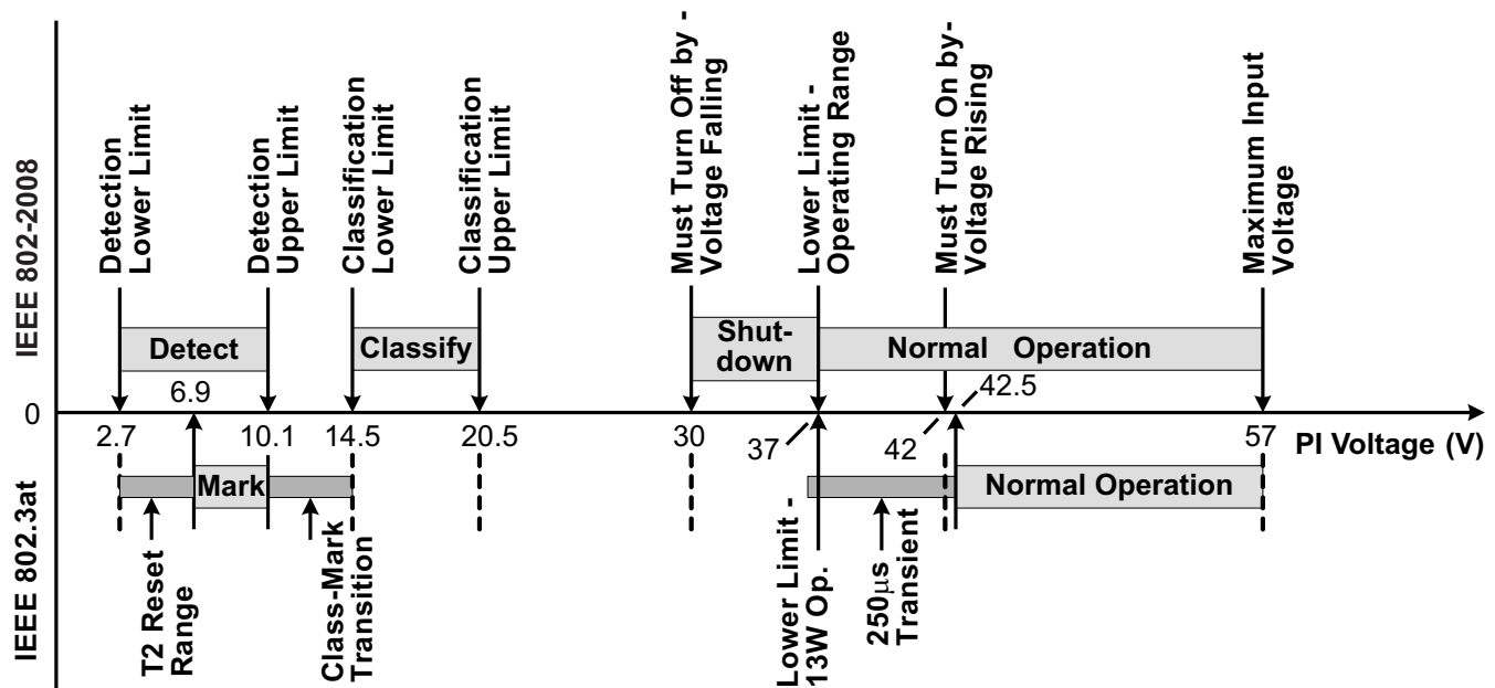
Figure 17. Threshold Voltages
