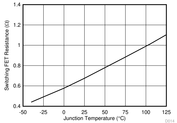
图 6-22. Switching FET Resistance vs Temperature
