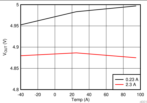
图 8-9. Output Regulation vs. Ambient Temperature
