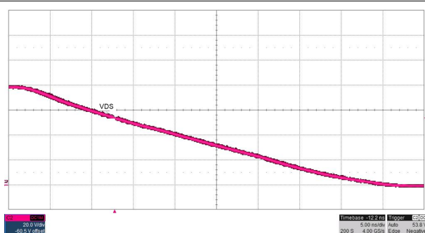
图 8-10. Slew Rate Adjust SRF = 100 Ω
