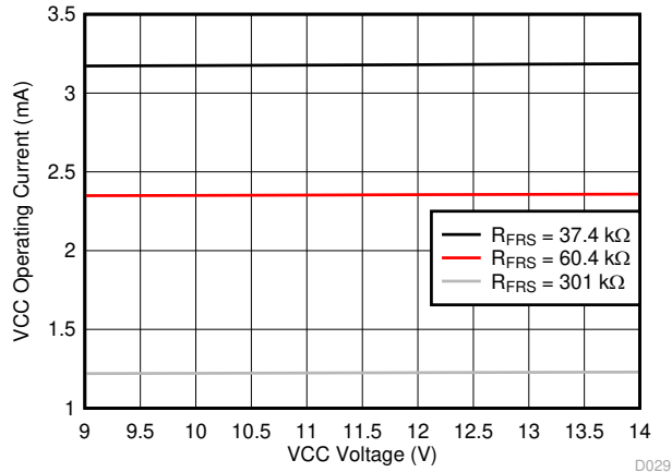
图 6-7. Controller Bias Current vs Voltage
