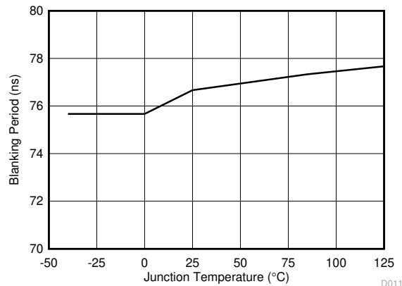
图 6-15. Blanking Period vs Temperature
