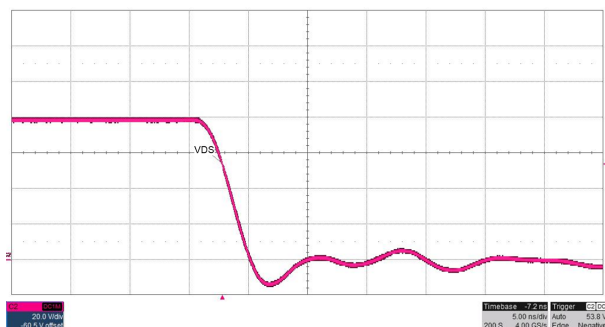
图 8-8. Slew Rate Adjust SRF = 0 Ω
