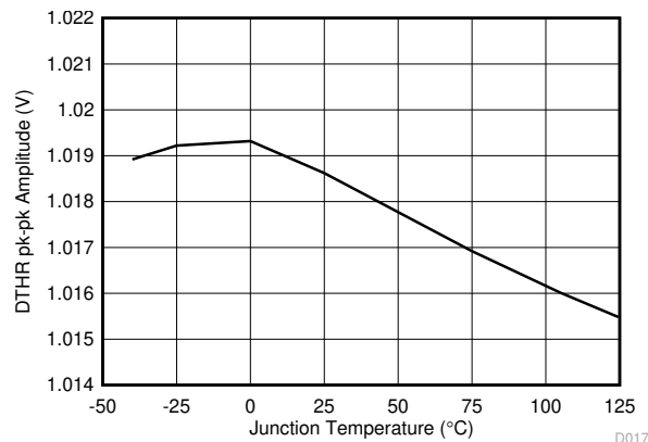
图 6-12. Frequency Dithering Peak-to-Peak Amplitude
