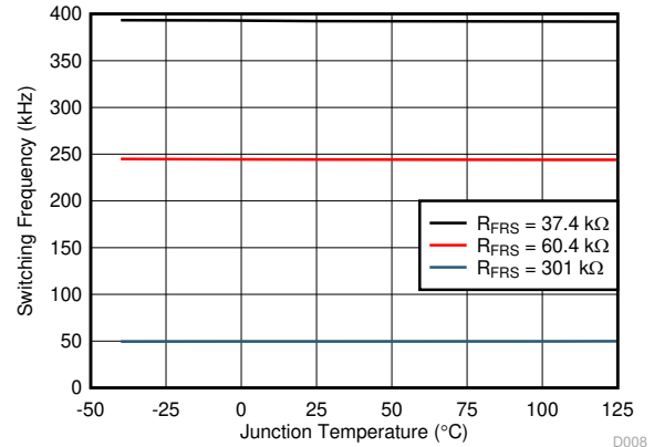
图 6-8. Switching Frequency vs Temperature
