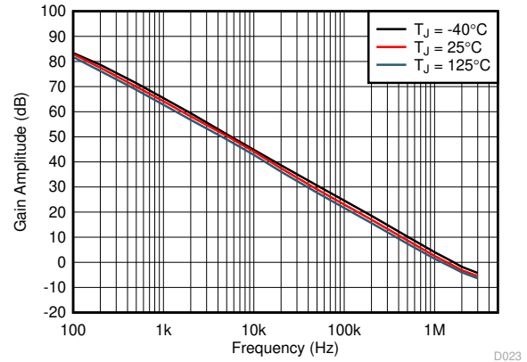
图 6-20. Error Amplifier Gain vs Frequency
