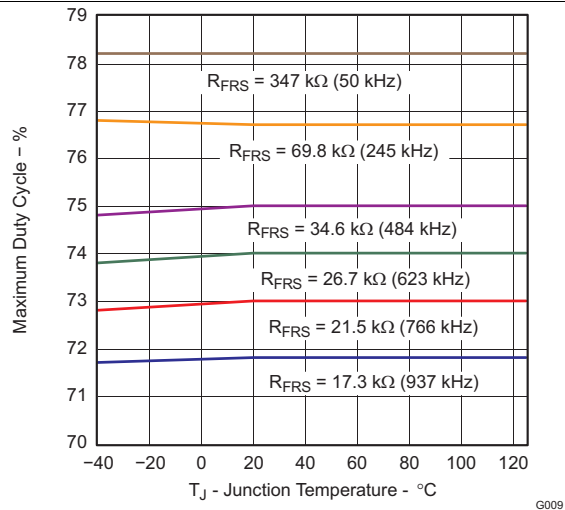
Figure 13. Maximum Duty Cycle vs Temperature
