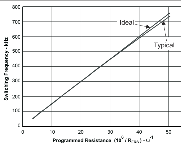
图 7-8. Switching Frequency vs Programmed Resistance
