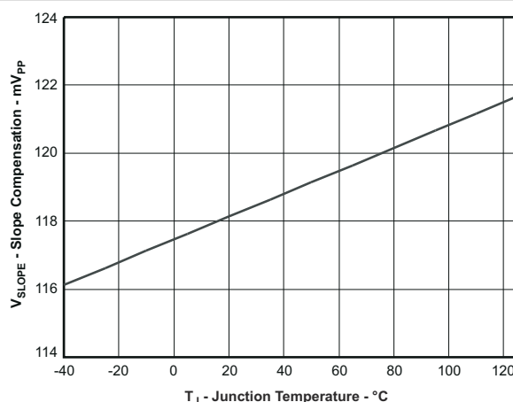
图 7-10. Current Slope Compensation Voltage vs Temperature
