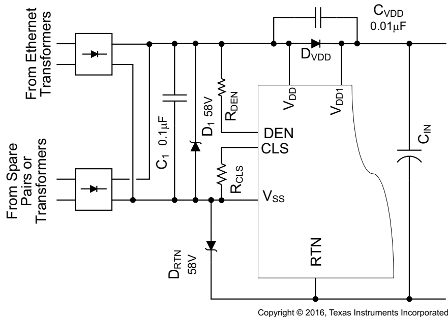
图 8-10. Additional Protection Against ESD
