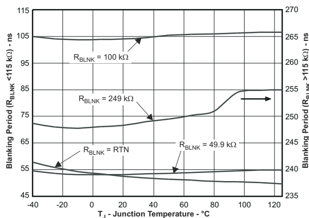
图 7-12. Blanking Period vs Temperature
