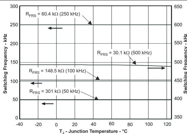
图 7-7. Switching Frequency vs Temperature
