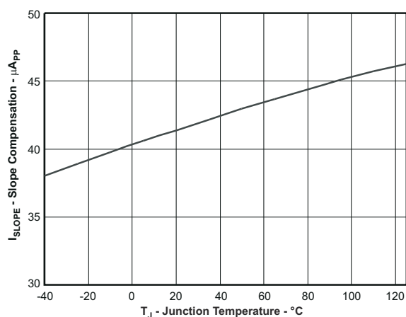
图 7-11. Current Slope Compensation Current vs Temperature
