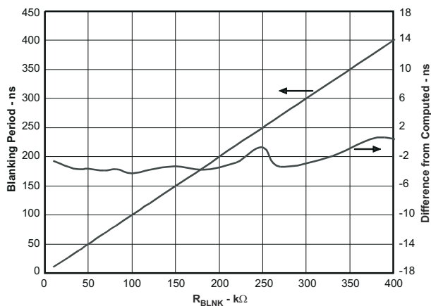
图 7-13. Blanking Period vs RBLNK
