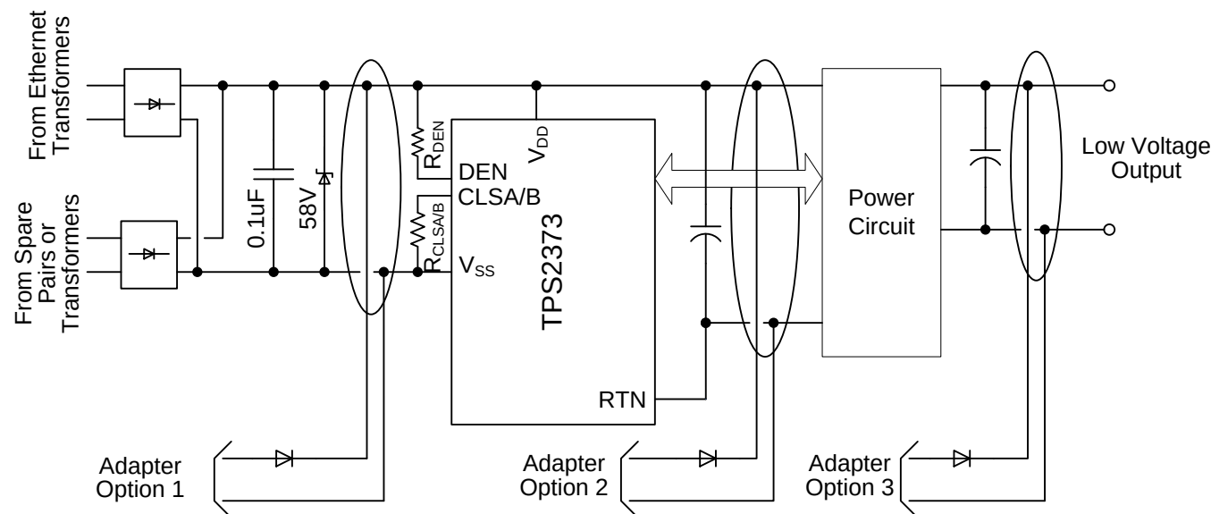
Figure 29. Oring 配置
