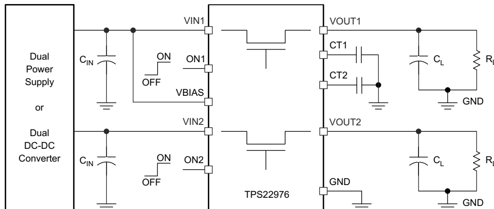
图 9-5. Typical Application Circuit
