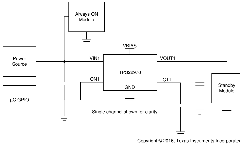
图 9-2. Standby Power Reduction
