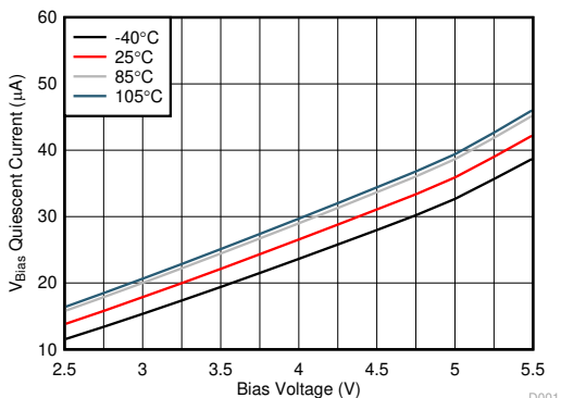
图 6-1. V_{BIAS} Quiescent Current vs Bias Voltage Both Channels (TPS22976, TPS22976N)
