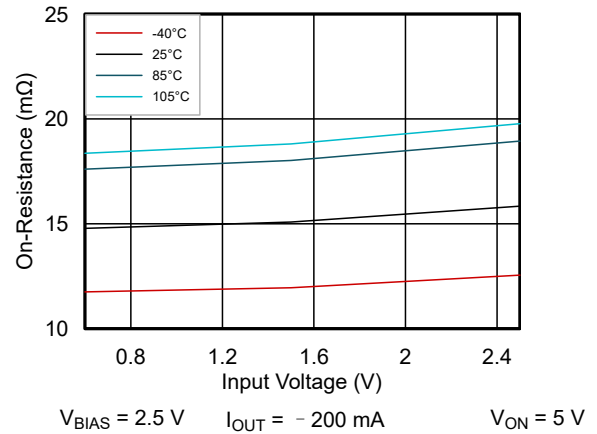
图 6-8. On-Resistance vs Input Voltage Single Channel - Across Ambient Temperatures (TPS22976)
