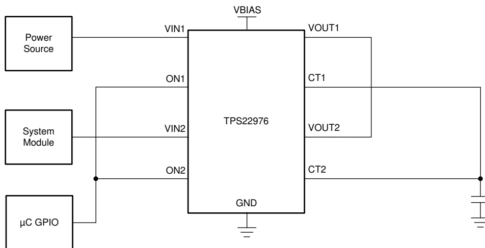
图 9-4. Reverse Current Blocking
