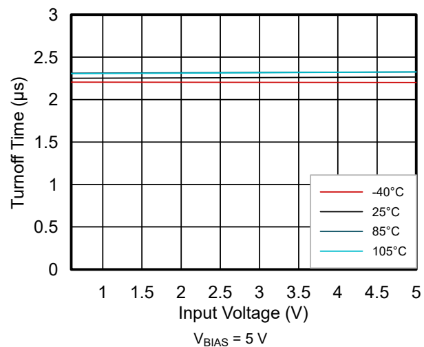
图 6-24. Turnoff Time vs Input Voltage (TPS22976)
