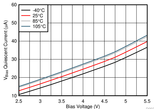
图 6-2. V_{BIAS} Quiescent Current vs Bias Voltage Single Channel (TPS22976, TPS22976N)
