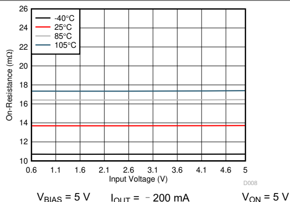
图 6-14. On-Resistance vs Input Voltage Single Channel - Across Ambient Temperatures (TPS22976A, TPS22976N)
