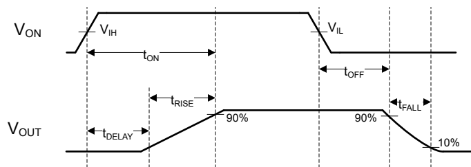
图 7-2. t_{ON} and t_{OFF} Waveforms
