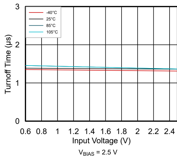
图 6-23. Turnoff Time vs Input Voltage (TPS22976)
