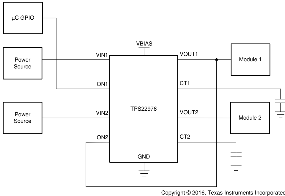
图 9-3. Power Sequencing without a GPIO Input
