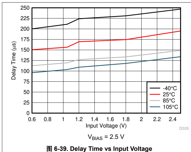
图 6-39. Delay Time vs Input Voltage
