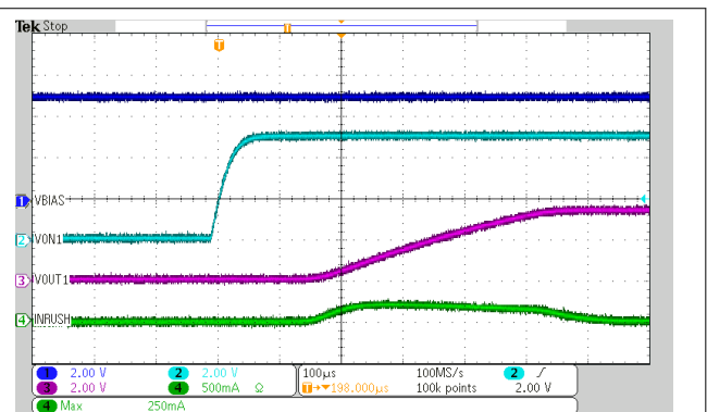
图 9-7. Inrush Current With CT = 220 pF
