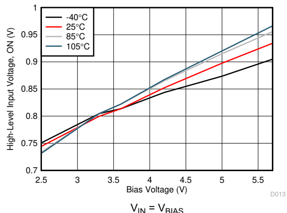
图 6-16. High-Level Input Voltage vs Bias Voltage
