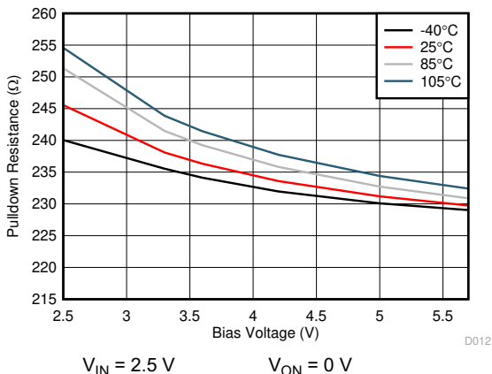
图 6-15. Pulldown Resistance vs Bias Voltage Single Channel
