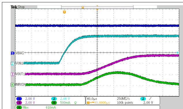
图 9-6. Inrush Current With CT = 0 pF
