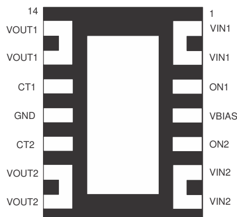
图 5-2. DPU Package 14-Pin WSON with Exposed Thermal Pad Bottom View
