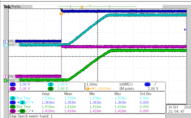
图 6-32. Turnon Response Time
