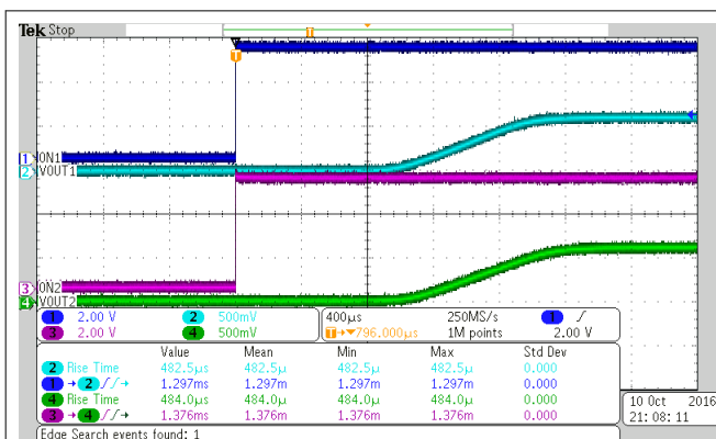
图 6-31. Turnon Response Time
