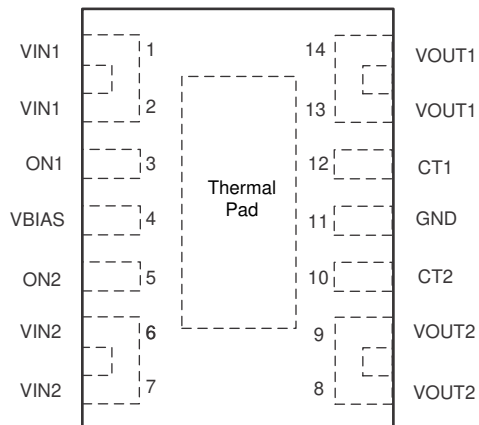
图 5-1. DPU Package 14-Pin WSON with Exposed Thermal Pad Top View
