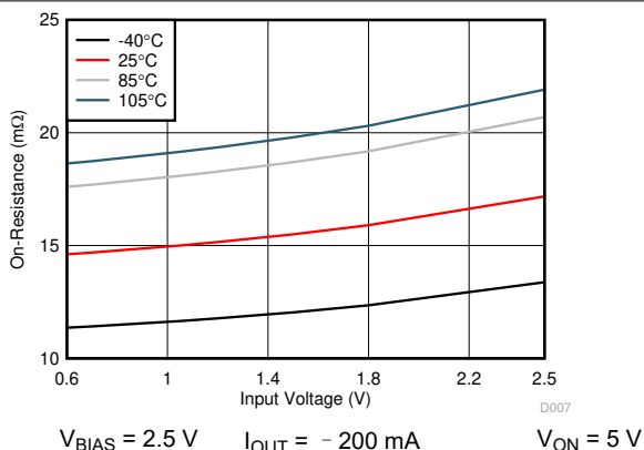
图 6-13. On-Resistance vs Input Voltage Single Channel - Across Ambient Temperatures (TPS22976A, TPS22976N)
