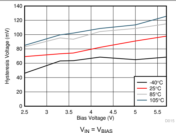
图 6-18. Voltage Input Hysteresis vs Bias Voltage
