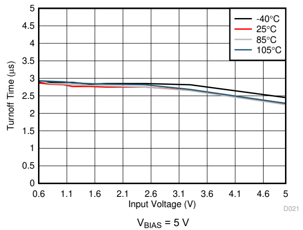
图 6-26. Turnoff Time vs Input Voltage (TPS22976N)
