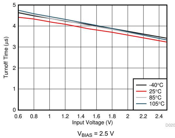
图 6-25. Turnoff Time vs Input Voltage (TPS22976N)
