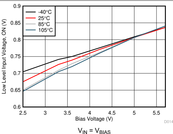
图 6-17. Low-Level Input Voltage vs Bias Voltage
