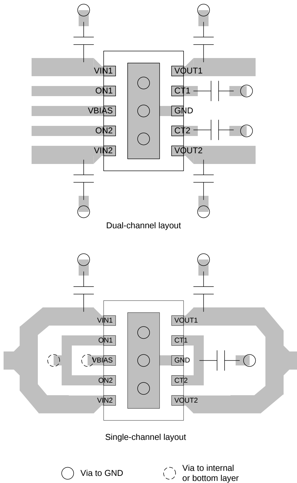
Figure 42. Layout Schematic
