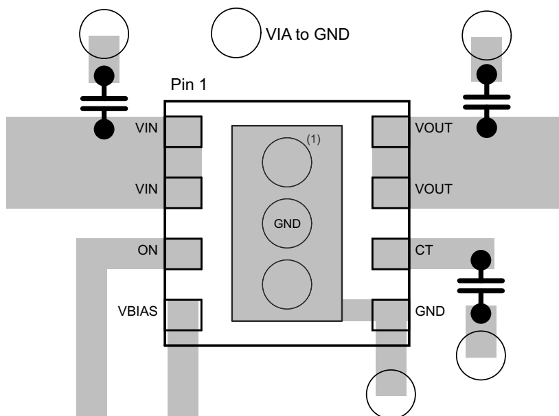
图 12-1. Layout Recommendation
