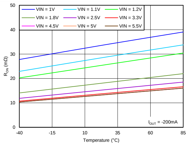
图 2. On Resistance vs Temperature
