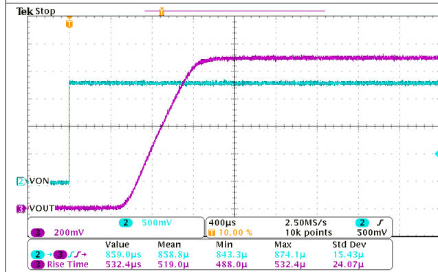
图 30. Turn-On Response Time ( V_{IN} = 1.2\text{ V} , C_{IN} = 1\text{ }\mu\text{F} , C_{OUT} = 0.1\text{ }\mu\text{F} , R_{OUT} = 10\text{ }\Omega )
