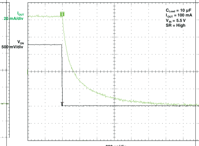
图 5-19. t_{OFF} Response
