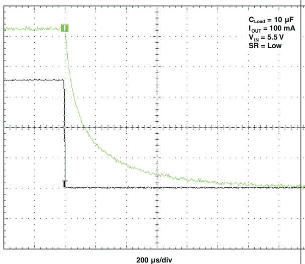
图 5-27. t_{OFF} Response
