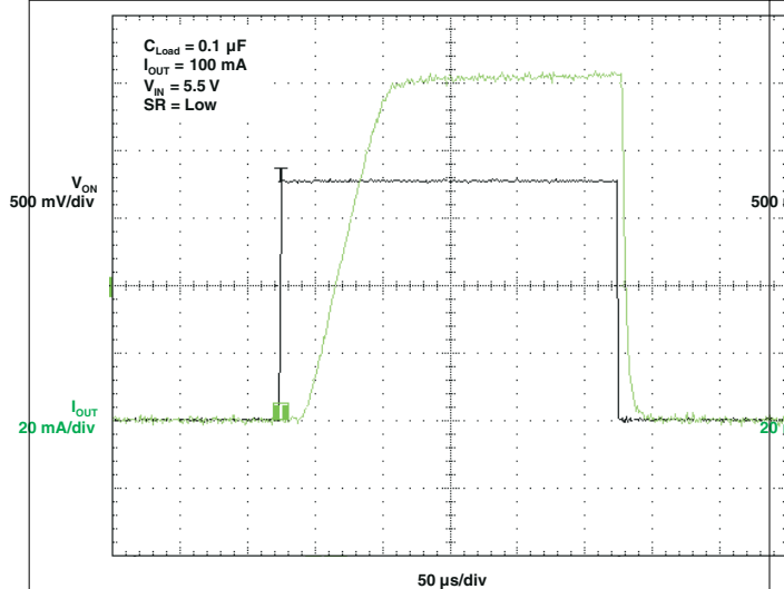
图 5-22. t_{ON} Response
