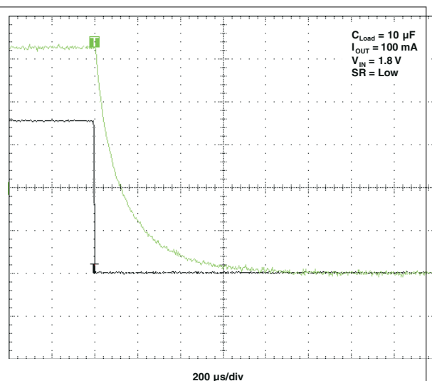
图 5-25. t_{OFF} Response
