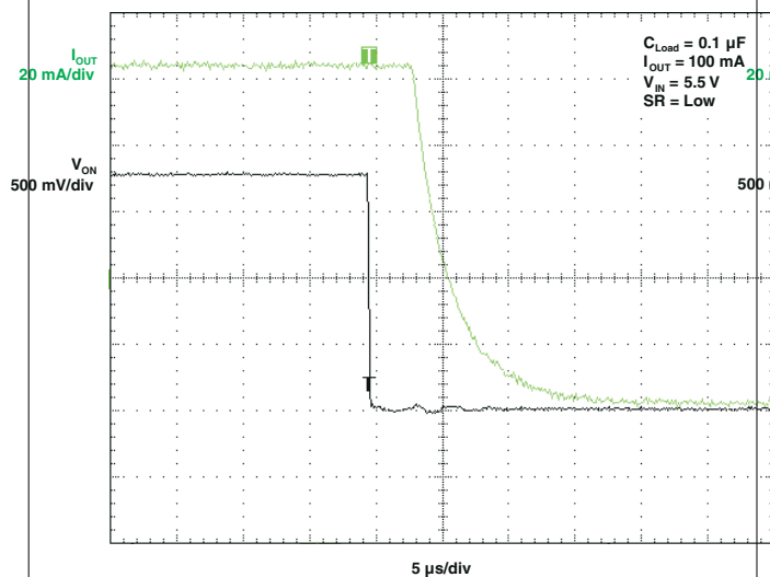
图 5-26. t_{OFF} Response
