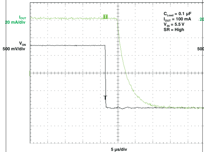
图 5-18. t_{OFF} Response
