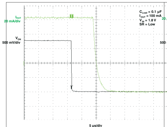
图 5-24. t_{OFF} Response
