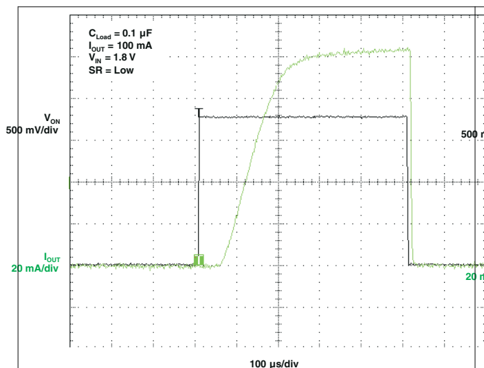
图 5-20. t_{ON} Response
