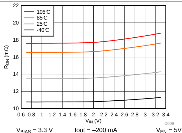
Figure 10. R_{ON} vs V_{IN} , V_{BIAS} = 3.3\text{ V}
