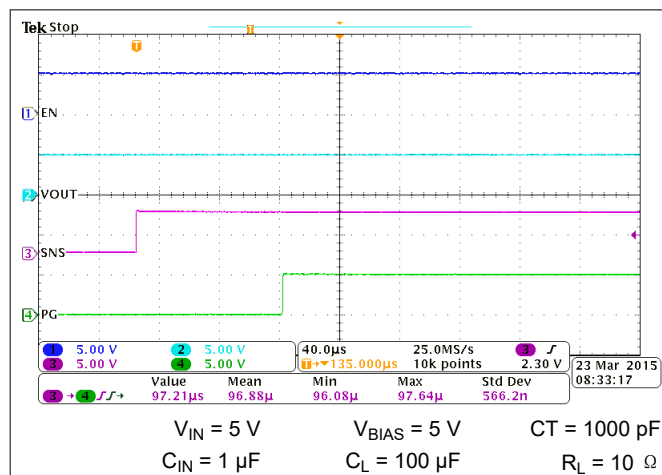
图 7-48. PG Response to SNS Rising ( t_{BLANK} )
