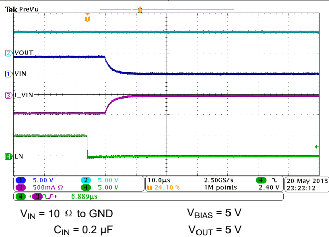
图 7-50. Reverse Current Blocking Response Time ( t_{RCB} )
