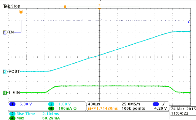
图 10-9. Inrush with CT = 470 pF
