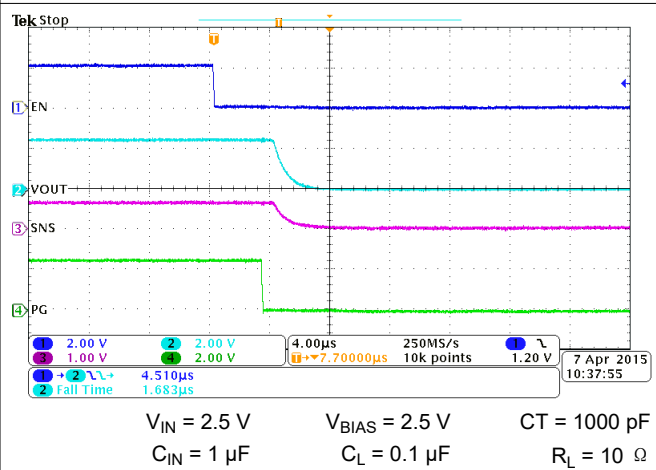
图 7-35. Turn-off Waveform, V_{BIAS} = 2.5\text{ V}
