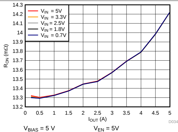
Figure 15. R_{ON} vs I_{OUT} , V_{BIAS} = 5\text{ V}
