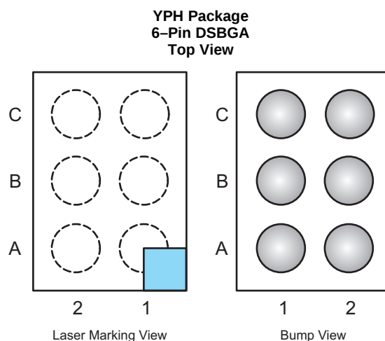
Pin Assignments
