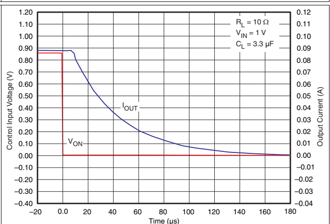
Figure 29. t_{OFF} Response
