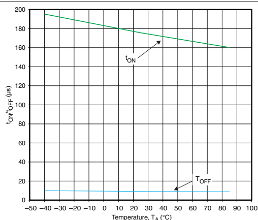
Figure 15. t ON /t OFF vs Temperature (V IN = 3.3 V)
