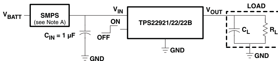
Figure 53. Typical Application
