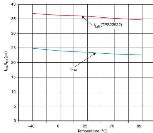
Figure 14. t rise /t fall vs Temperature (V IN = 3.3 V)
