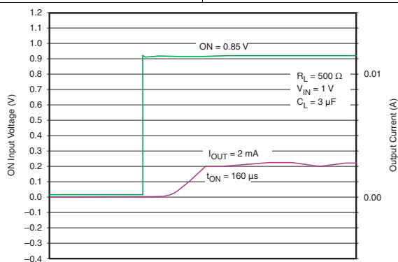
Figure 21. t_{ON} Response
