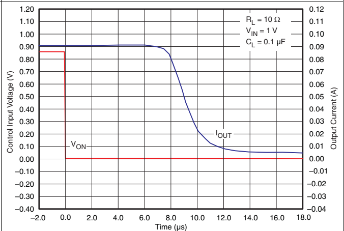
Figure 27. t_{OFF} Response
