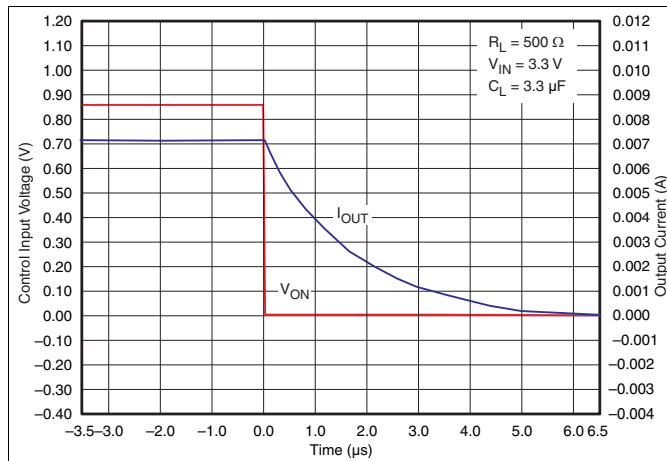
Figure 24. t_{OFF} Response
