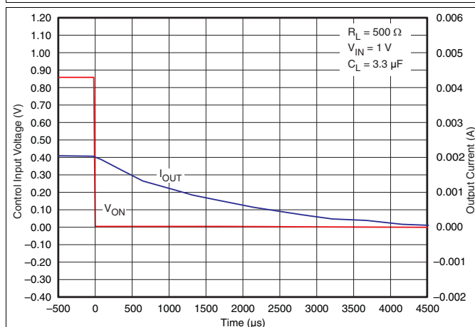
Figure 28. t_{OFF} Response
