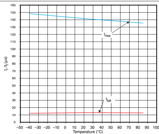
Figure 16. t rise /t fall vs Temperature (V IN = 3.3 V)
