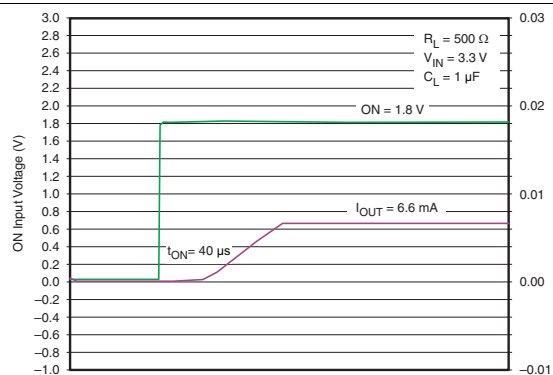
Figure 17. t ON Response
