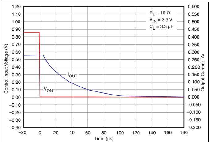
Figure 25. t_{OFF} Response
