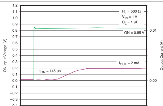
Figure 20. t_{ON} Response
