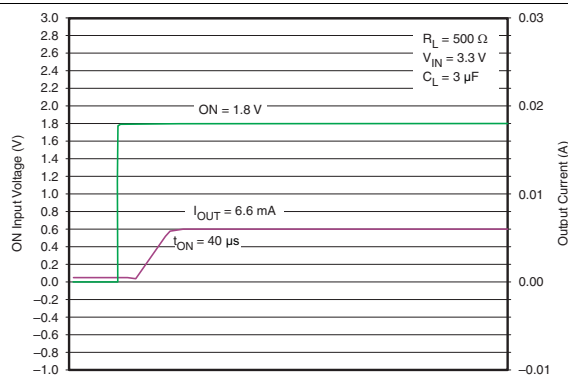
Figure 18. t ON Response
