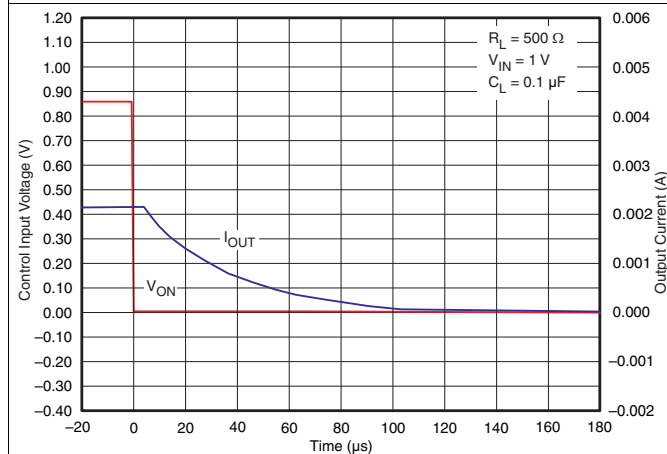
Figure 26. t_{OFF} Response
