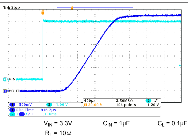
图 6-29. t_R = V_{IN} = 3.3V
