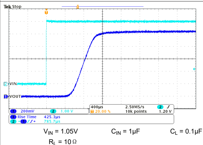
图 6-31. t_R = V_{IN} = 1.05V
