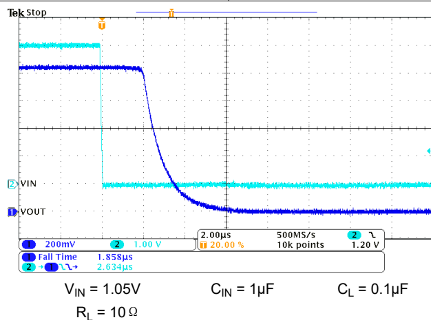
图 6-32. t_F = V_{IN} = 1.05V
