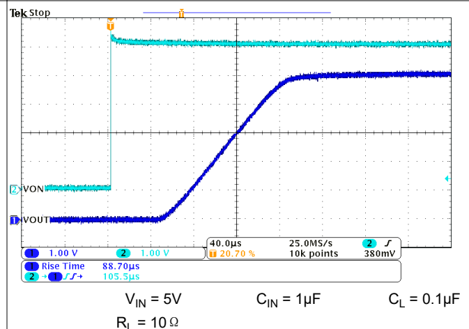
图 6-16. t_R = V_{IN} = 5V
