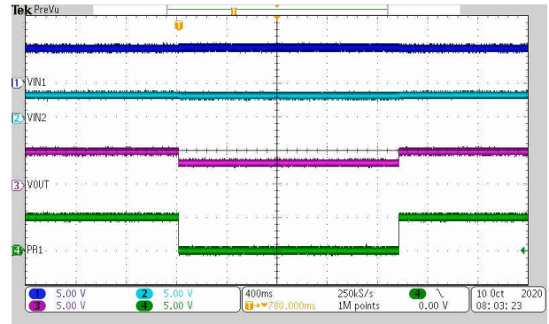
图 6-13. Manual Mode Switchover Behavior (MODE = 5 V, R_L = 10 \Omega , C_L = 10 \mu\text{F} )
