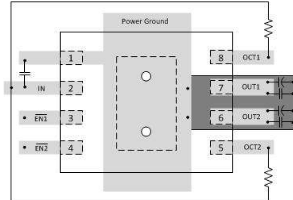
图 11-1. Layout Recommendation
