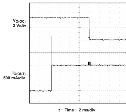
图 9-34. 2- \Omega Load Connected to Enabled Device
