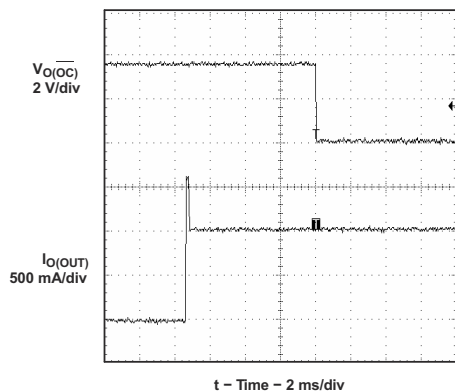
图 9-33. 3- \Omega Load Connected to Enabled Device
