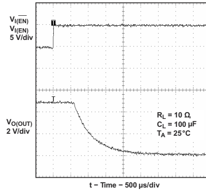
图 9-6. Turnoff Delay and Fall Time With 100-μF Load
