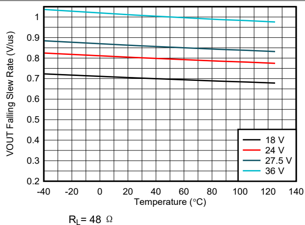
图 6-12. VOUT Falling Slew Rate ( SR_F ) vs Temperature vs VS Voltage
