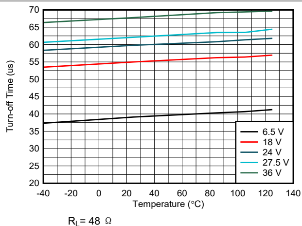
图 6-10. Turn-off Time ( t_{OFF} ) vs Temperature vs VS Voltage
