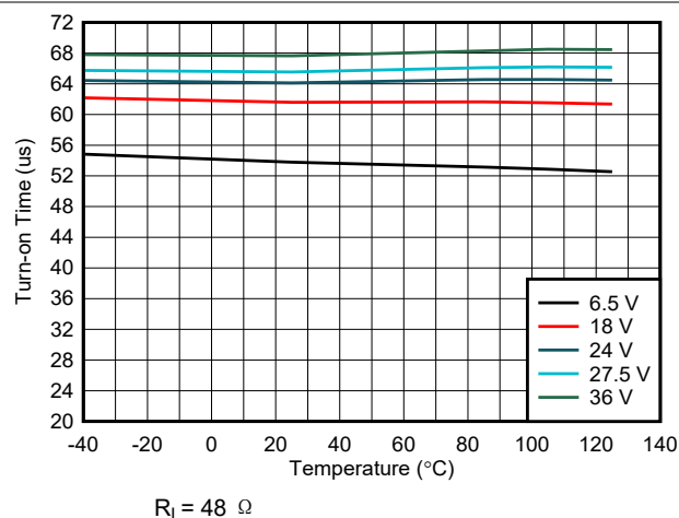
图 6-9. Turn-on Time ( t_{ON} ) vs Temperature vs VS Voltage
