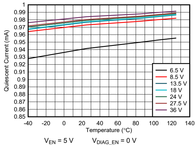
图 6-5. Quiescent Current ( I_{Q, VS} ) From VS Input Supply vs Temperature vs VS Voltage
