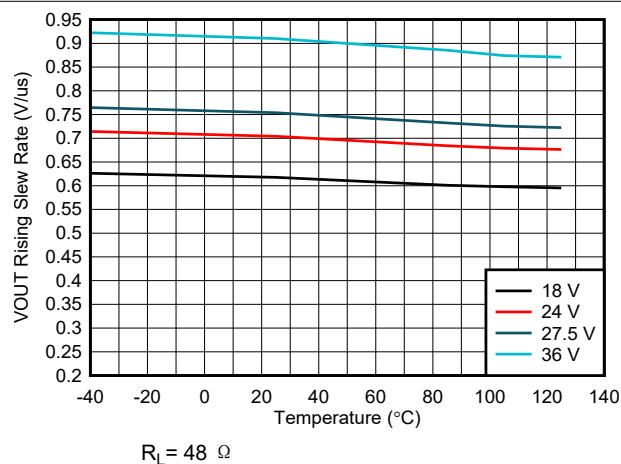
图 6-11. VOUT Rising Slew Rate ( SR_R ) vs Temperature vs VS Voltage
