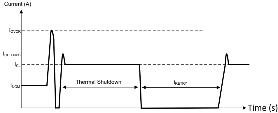
图 8-8. On-State Short-Circuit Behavior
