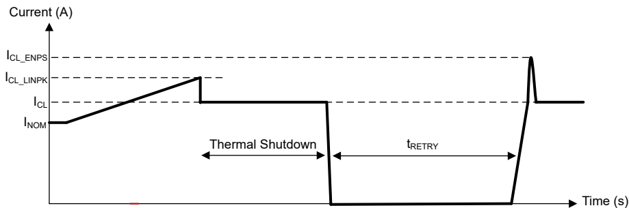
Figure 7-7. Overload Behavior
