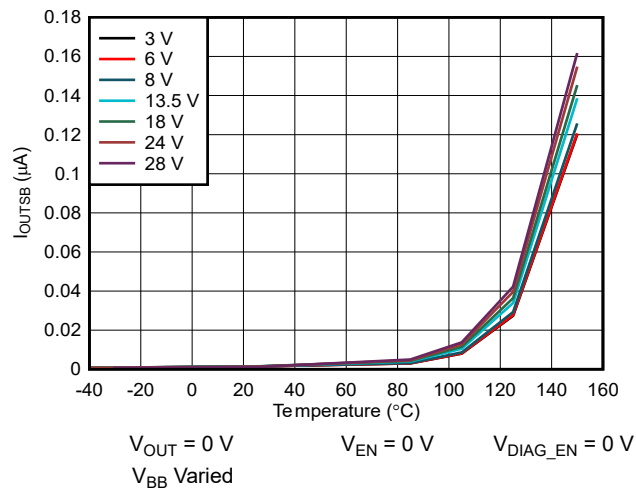
图 5-3. Output Leakage Current I_{OUT,STBY} vs Temperature
