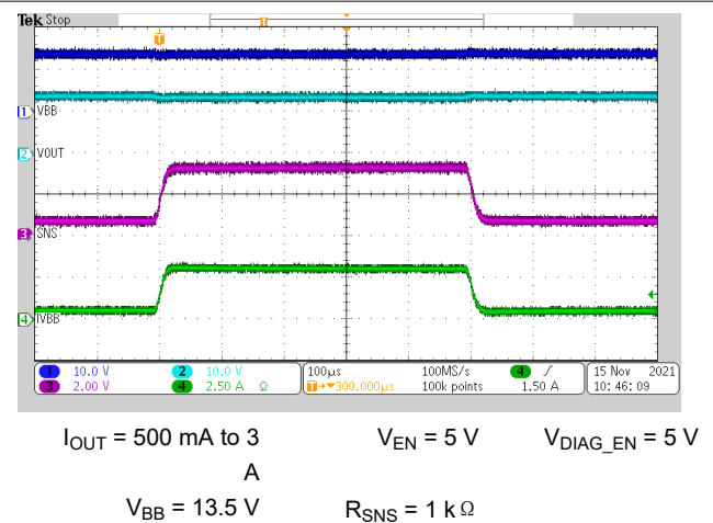
图 5-22. ISNS Settling Time ( t_{SNSION} ) on Load Step
