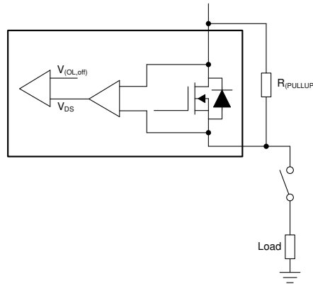
图 7-10. Open-Load Detection in Output OFF State
