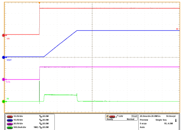
图 9-3. Inrush Current Control for Hot Plugin at Input
