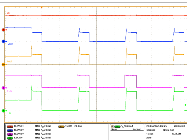
图 8-13. Power Limiting ( I_{OCP} \leq I_{OUT} < I_{fast-trip} )
