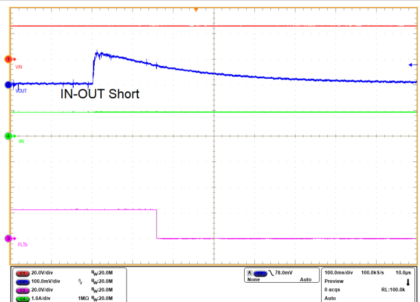
图 9-7. IN to OUT Short Detection with V_{IN} = 24\text{ V}
