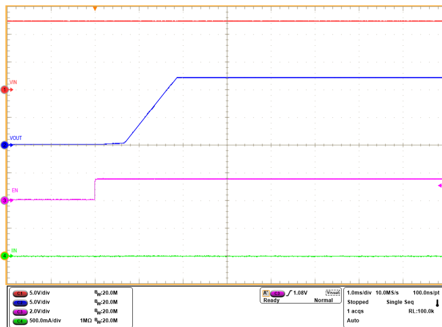
图 8-1. EN/SHDN in TPS1641x Devices
