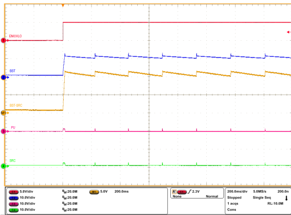
图 9-2. INP1=INP2 = GND 且 C_{BST} = 470nF 时自举电压的启动曲线
