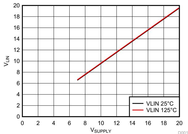
图 7-2. V_{OH} vs V_{SUPPLY} and Temperature
