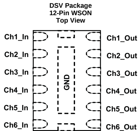
Pin Functions
