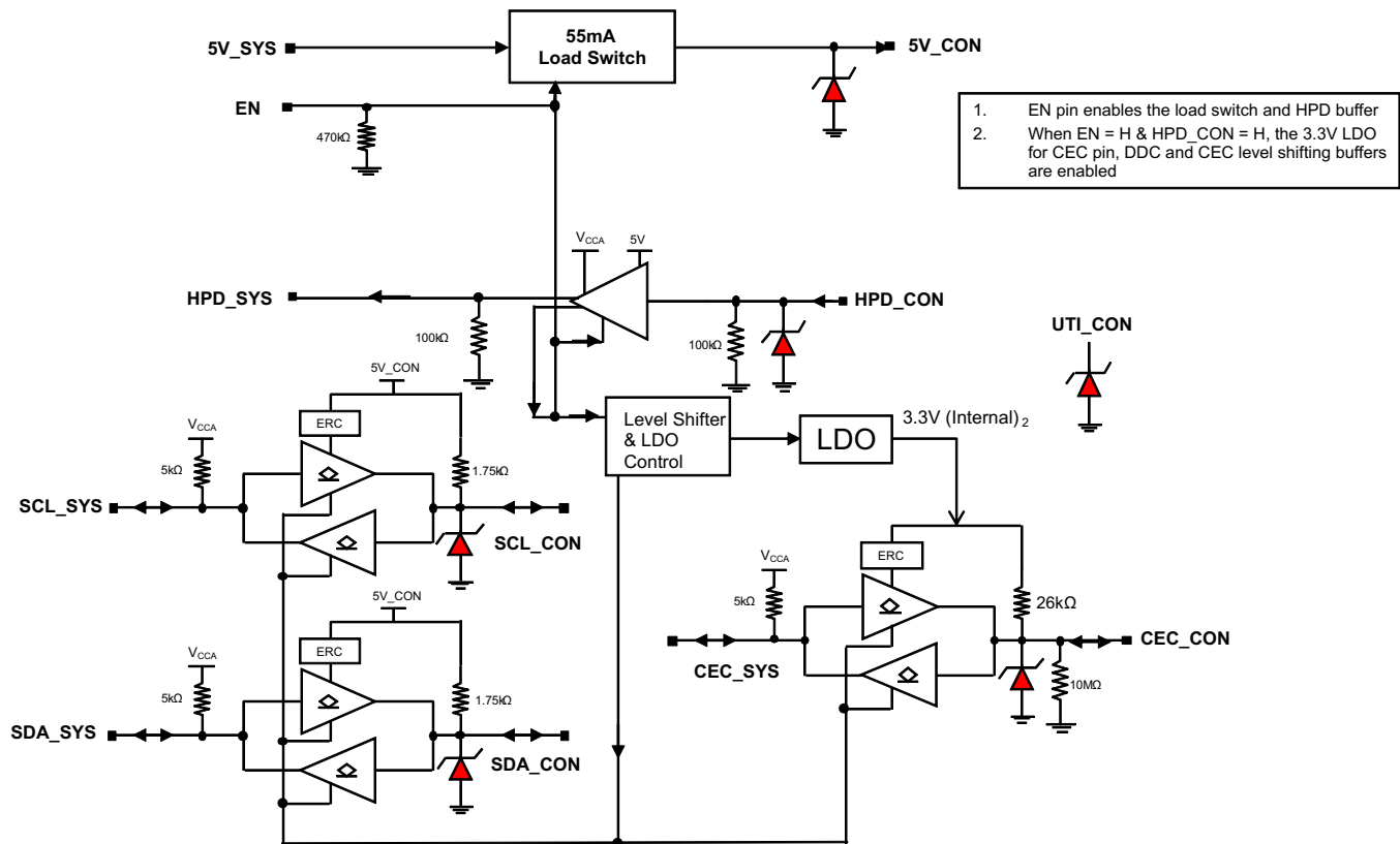
Figure 1. Circuit Schematics
