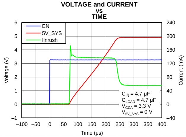
Figure 16. I_{INRUSH} Waveform Data
