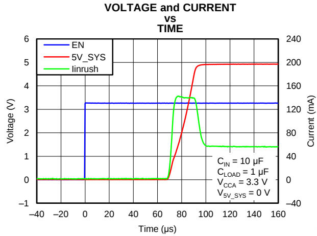
Figure 15. I_{INRUSH} Waveform Data
