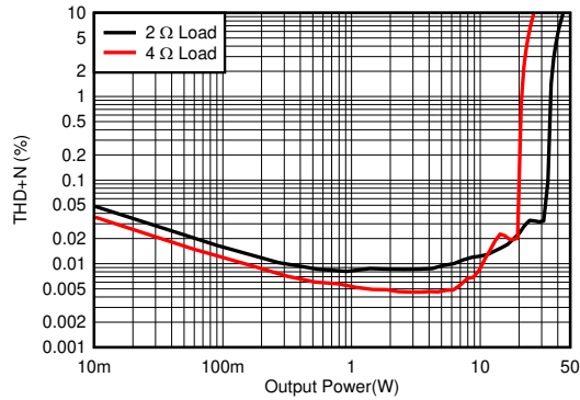
图 6-1. THD+N vs Power - 2 \Omega , 4 \Omega - 14.4 V
