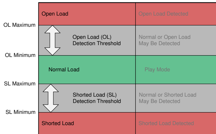
图 7-3. DC Load Diagnostic Reporting Thresholds
