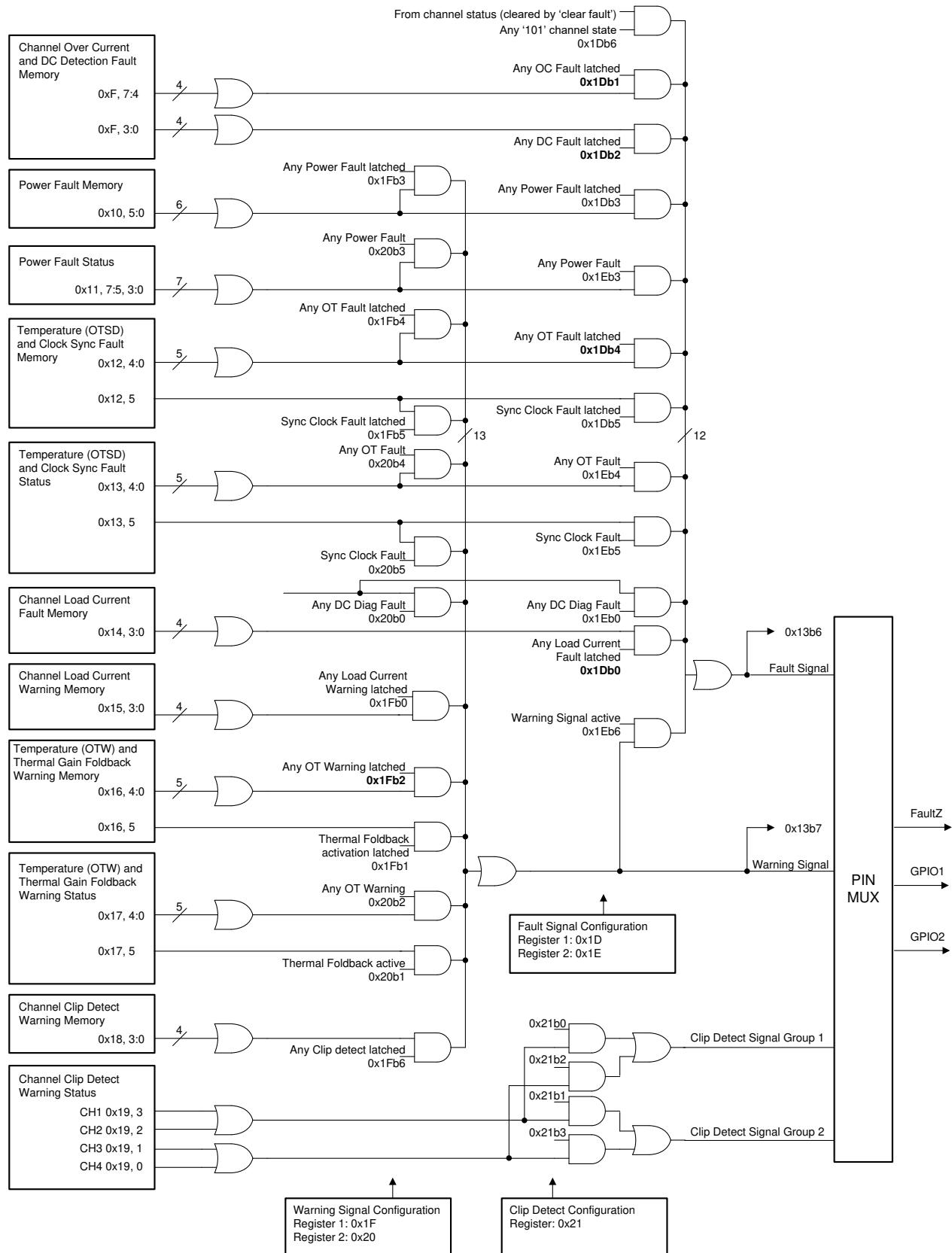
图 7-7. Fault, Warning and Clip Detect Signal Creation and Configuration
