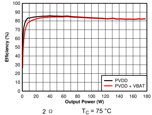
图 6-56. Efficiency vs Output Power - 2 \Omega
