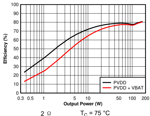
图 6-9. Efficiency vs Output Power - 2 Ω (Zoomed)
