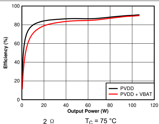
图 6-22. Efficiency vs Output Power - PBTL, 2 Ω
