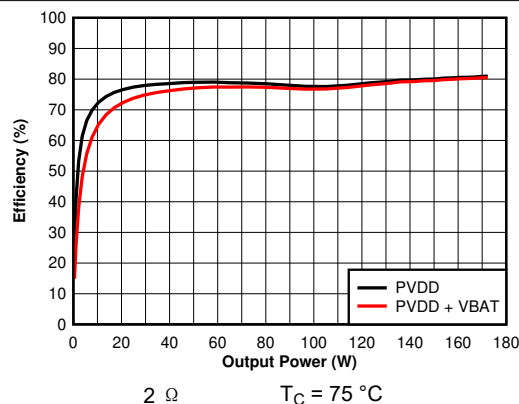
图 6-8. Efficiency vs Output Power - 2 Ω
