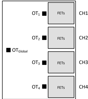
图 7-5. Temperature Sensor Locations Within the Device
