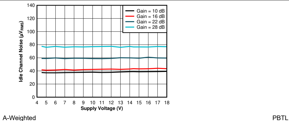
图 6-24. Noise vs Supply Voltage - PBTL, 2 Ω
