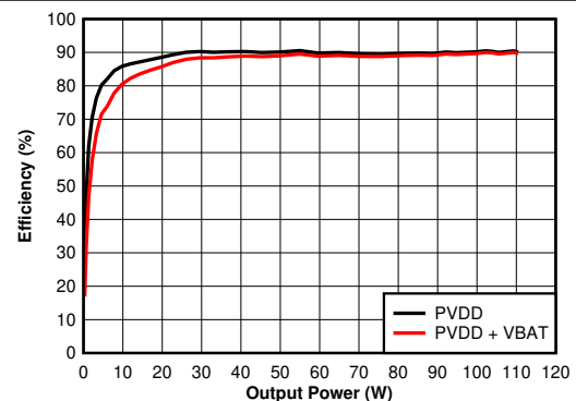
图 6-41. Efficiency vs Output Power - 4 \Omega
