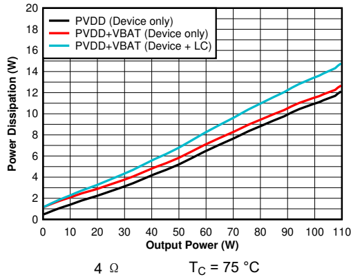
图 6-55. Power Dissipation vs Output Power - 4 \Omega
