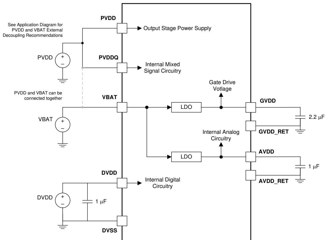
图 9-1. Power Supply Block
