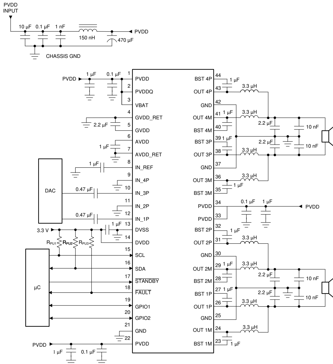
图 8-3. 2-Channel PBTL Application Schematic
