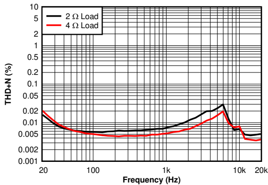
图 6-3. THD+N vs Frequency - 2 \Omega , 4 \Omega
