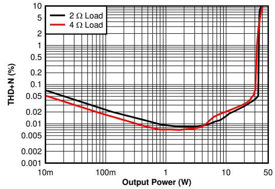
图 6-26. THD+N vs Power - BTL, 2 Ω, 4 Ω, 18 V, 1SPW
