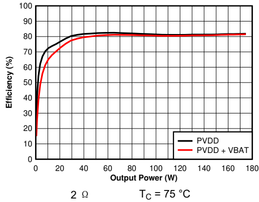
图 6-31. Efficiency vs Output Power - BTL, 2 \Omega , 14.4 V, 1SPW
