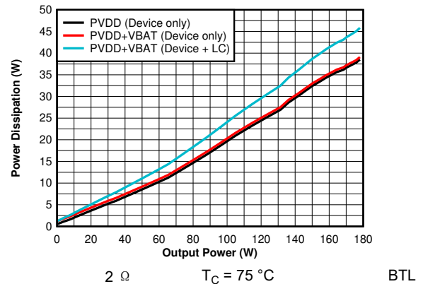
图 6-58. Power Dissipation vs Output Power - 2 \Omega
