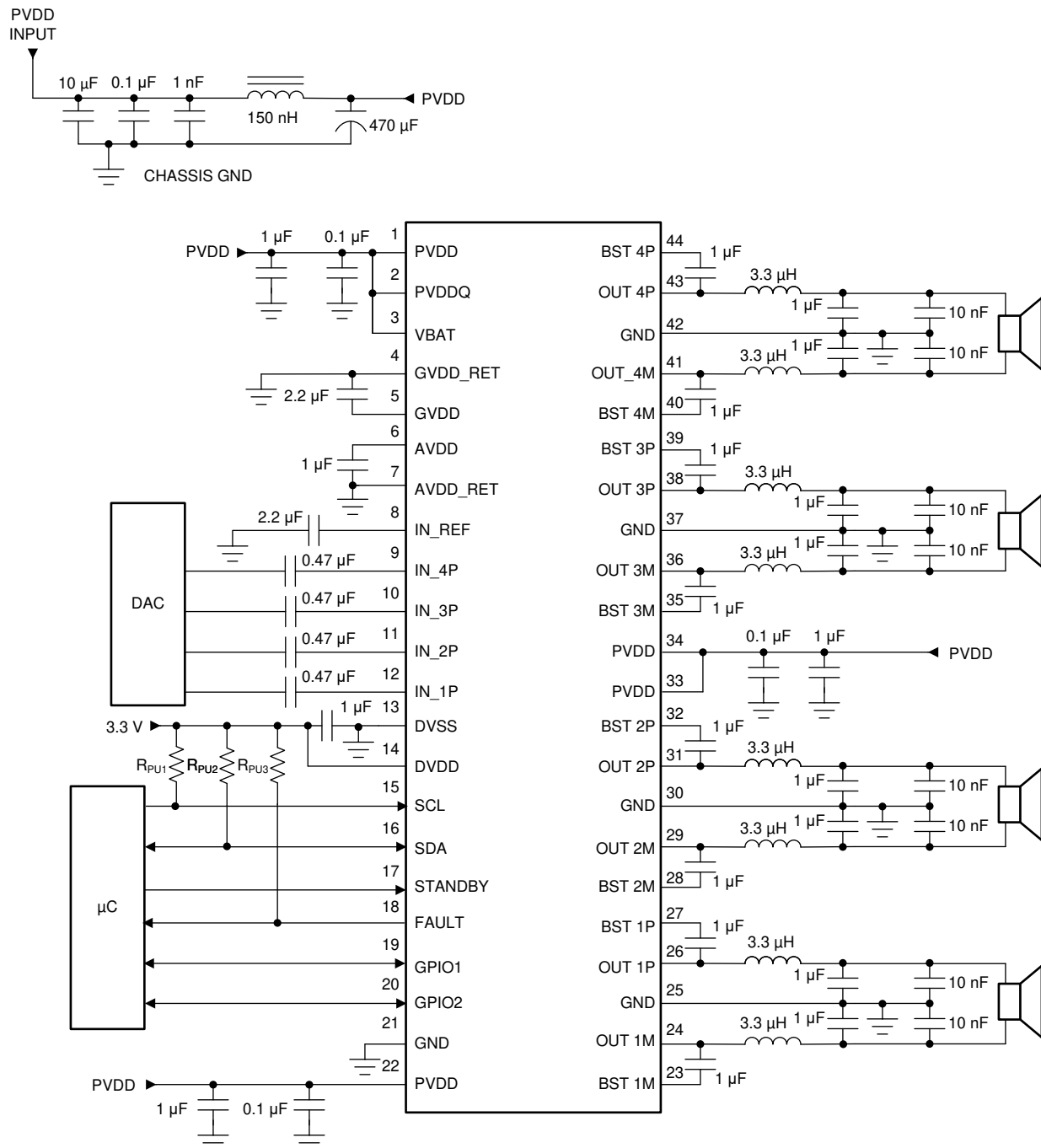
图 8-2. Typical 4-Channel BTL Application Schematic
