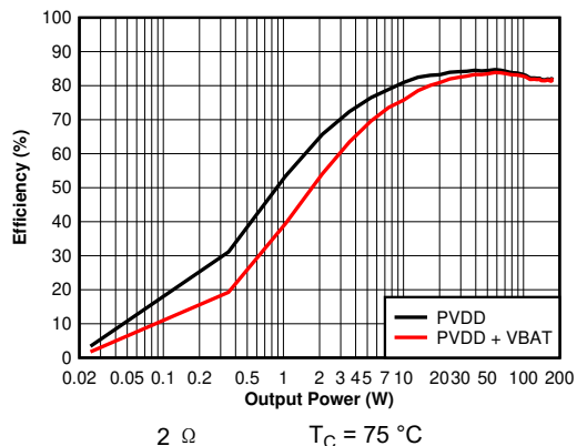
图 6-45. Efficiency vs Output Power - 2 \Omega (Zoomed)
