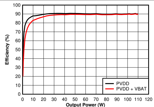
图 6-53. Efficiency vs Output Power - 4 Ω
