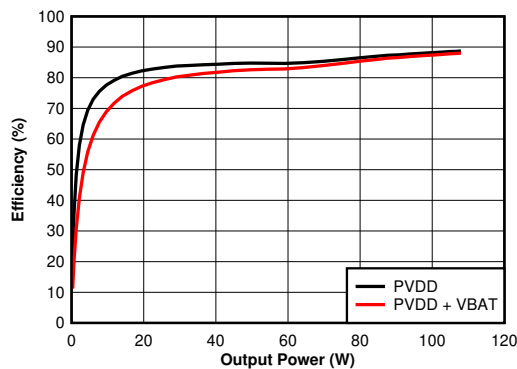
图 6-5. Efficiency vs Output Power - 4 \Omega
