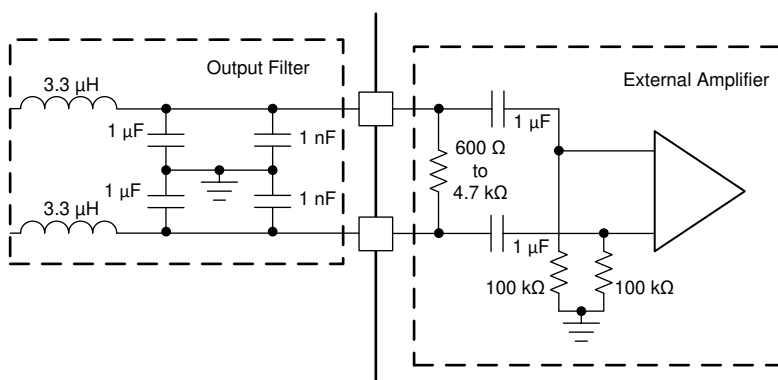
图 8-1. Line Driver External Amplifier Input Configuration
