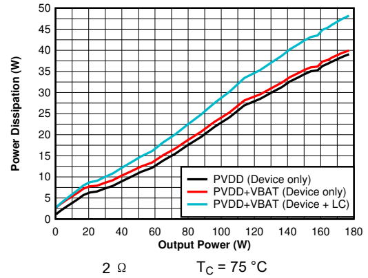
图 6-32. Power Dissipation vs Output Power - BTL, 2 \Omega , 14.4 V, 1SPW
