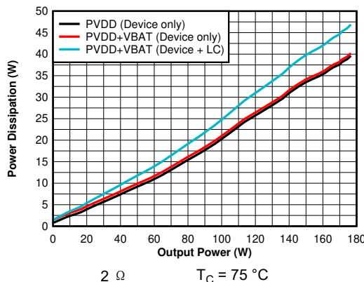
图 6-46. Power Dissipation vs Output Power - 2 \Omega
