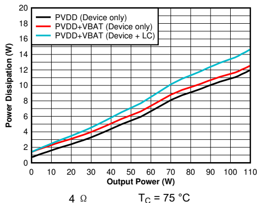
图 6-43. Power Dissipation vs Output Power - 4 \Omega
