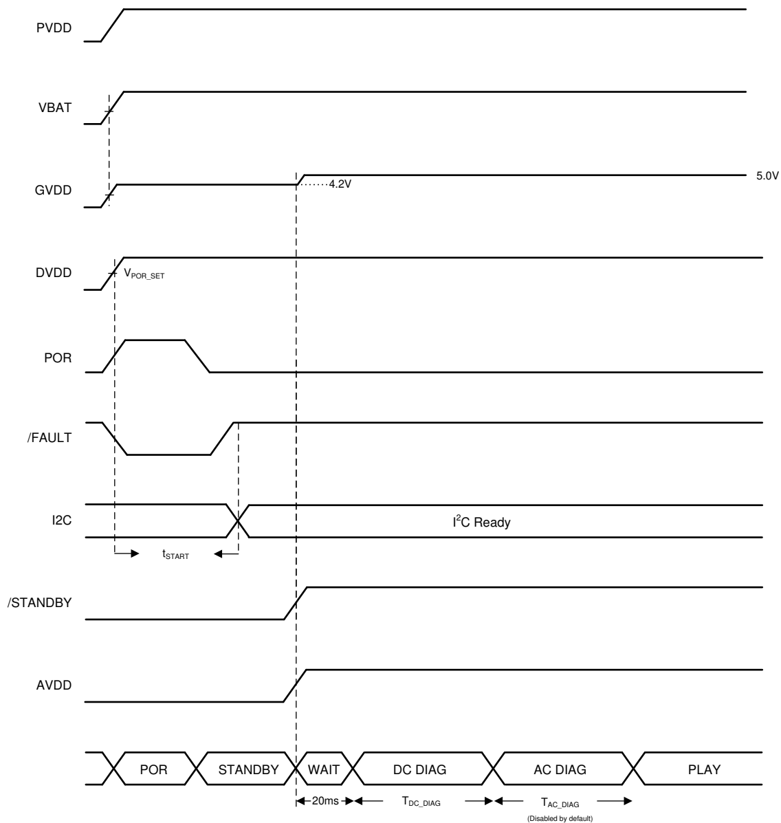
图 7-4. Typical Initialization Sequence and Timing
