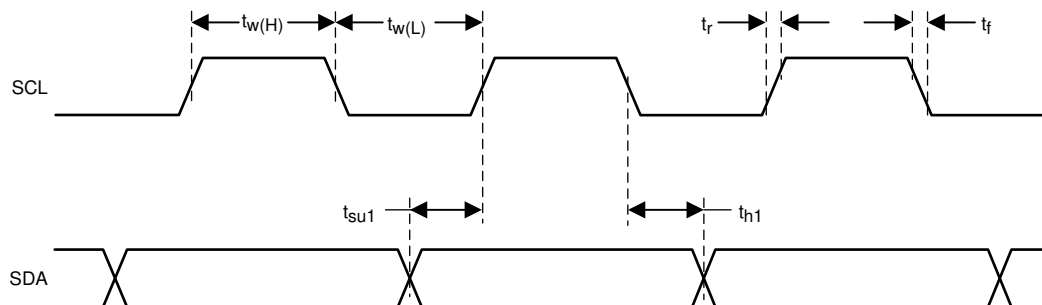
图 7-9. SCL and SDA Timing
