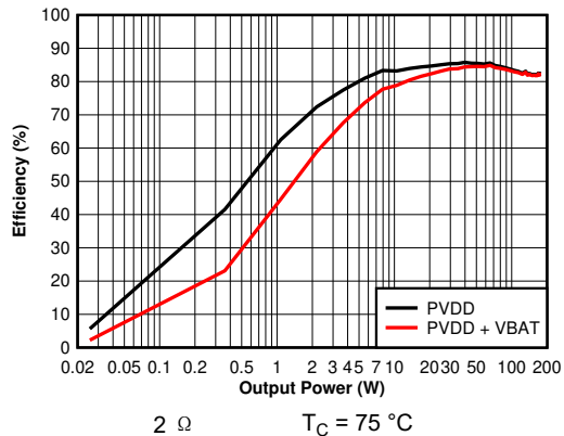
图 6-57. Efficiency vs Output Power - 2 \Omega (Zoomed)
