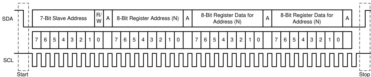
图 7-8. Typical I 2 C Sequence
