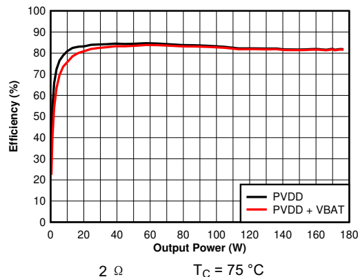
图 6-44. Efficiency vs Output Power - 2 \Omega
