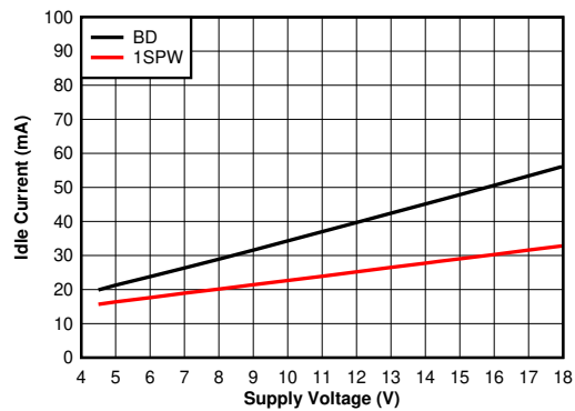
图 6-33. PVDD Idle Current vs Supply Voltage - BTL, 1SPW
