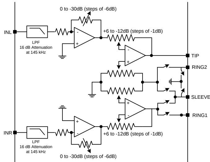
Figure 28. Audio Playback Channel
