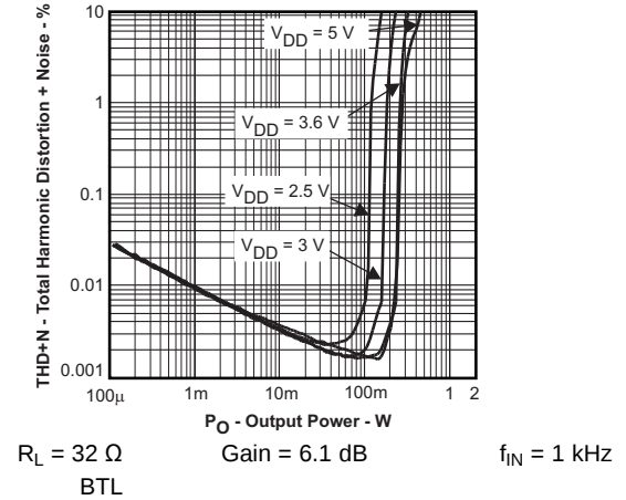
Figure 8. Total Harmonic Distortion + Noise vs Output Power
