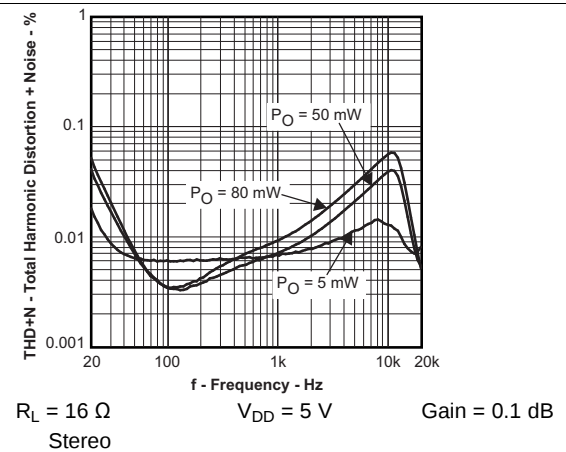
Figure 12. Total Harmonic Distortion + Noise vs Frequency
