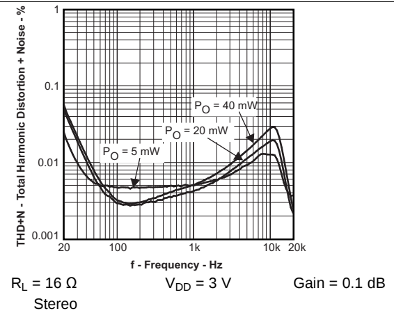
Figure 10. Total Harmonic Distortion + Noise vs Frequency
