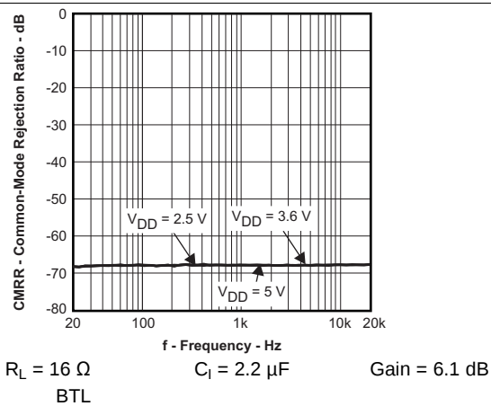
Figure 27. Common Mode Rejection Ratio vs Frequency
