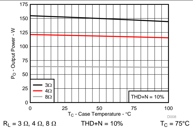
图 8. Output Power vs Case Temperature
