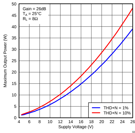
图 13. Maximum Output Power (BTL) vs Supply Voltage
