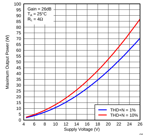
图 14. Maximum Output Power (BTL) vs Supply Voltage
