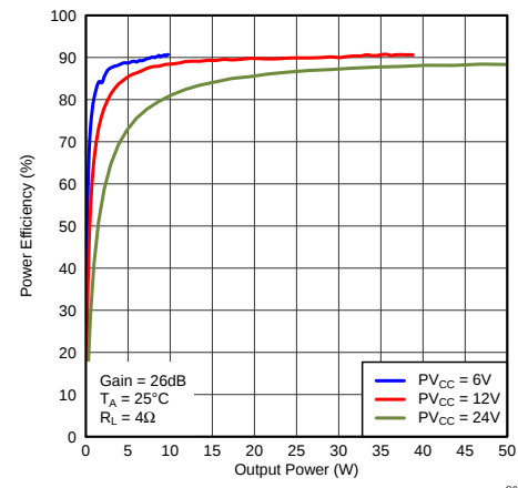
图 16. Power Efficiency (BTL) vs Output Power
