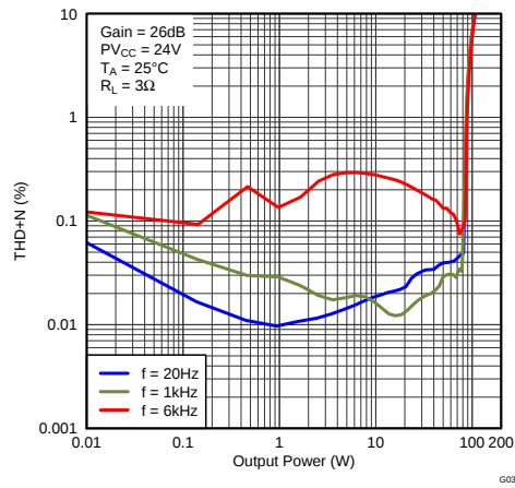
图 25. Total Harmonic Distortion + Noise (PBTL) vs Output Power
