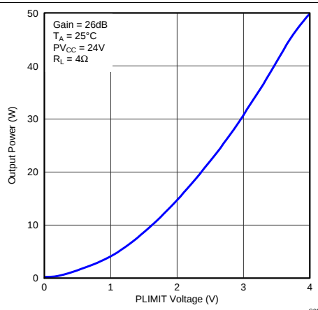
图 11. Output Power (BTL) vs Plimit Voltage
