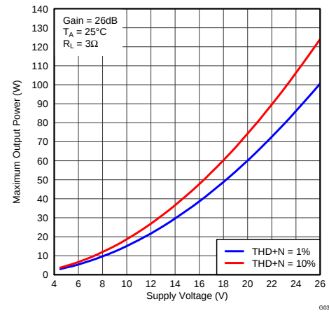
图 26. Maximum Output Power (PBTL) vs Supply Voltage
