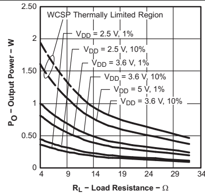
Figure 33. Output Power vs Load Resistance
