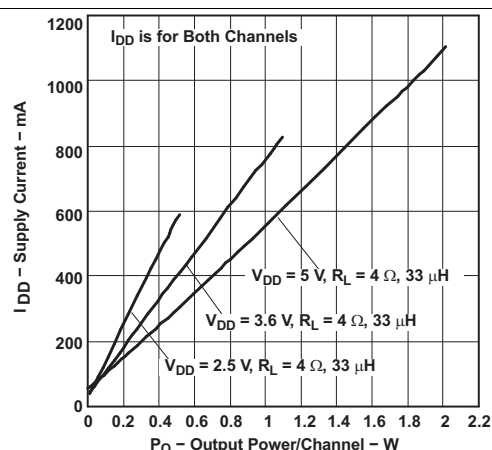
Figure 14. Supply Current vs Output Power
