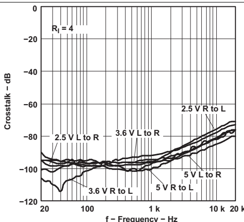
Figure 16. Crosstalk vs Frequency
