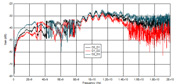
图 5-8. 公共端口侧通道之间的串扰 (Xtalk)
