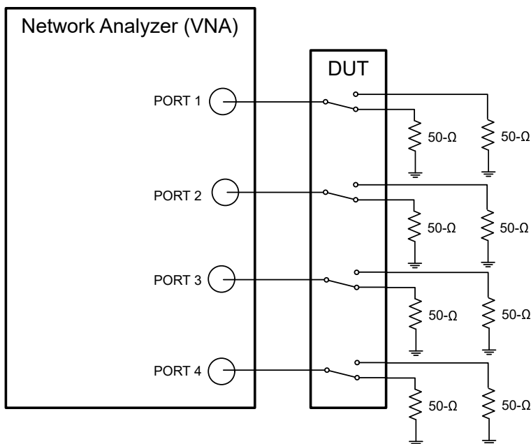
图 6-4. 串扰 (Xtalk)
