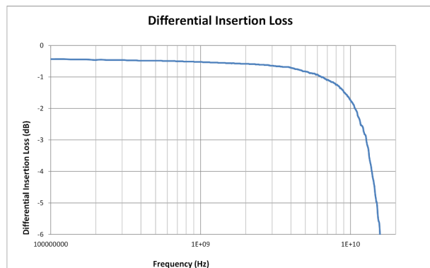
图 5-1. S-Parameter Plots for a TMUXHS4412 Channel: Differential Insertion Loss
