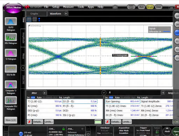
图 5-6. Jitter Decomposition of 20Gbps PRBS-7 Signals in TI Evaluation Board Through a Typical TMUXHS4412 Channels
