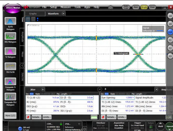
图 5-3. Jitter Decomposition of 10Gbps PRBS-7 Signals in TI Evaluation Board Through Calibration Traces
