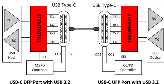
USB-C DFP Port with USB 3.2
