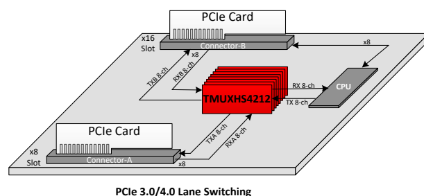
PCIe 3.0/4.0 Lane Switching
