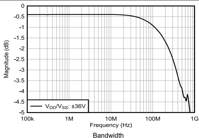
图 7-26. Insertion Loss vs Frequency
