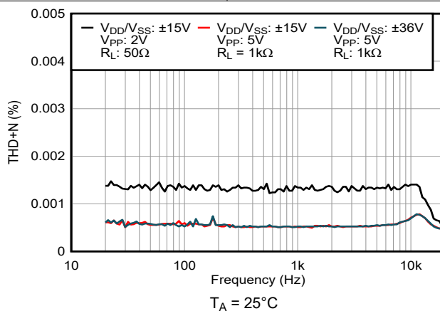
图 7-27. THD+N vs Frequency
