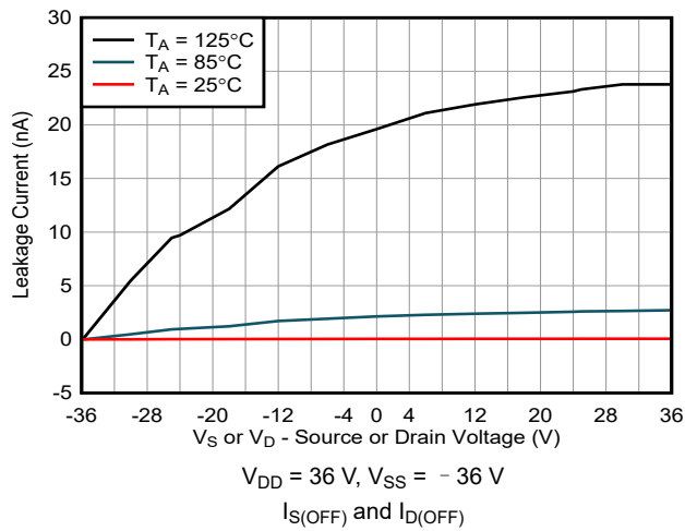
图 7-15. Off-Leakage Current vs Source or Drain Voltage
