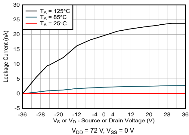
图 7-17. Off-Leakage Current vs Source or Drain Voltage
