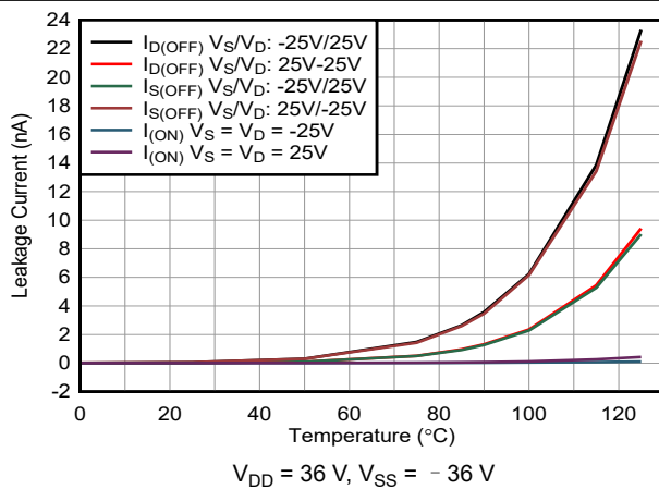
图 7-11. Leakage Current vs Temperature
