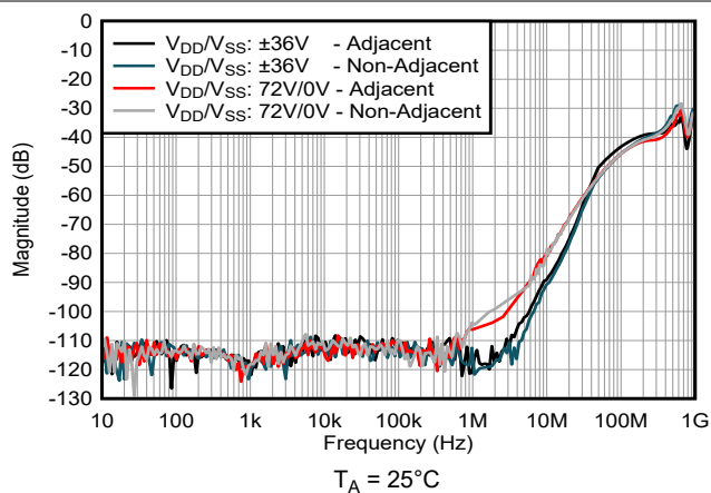
图 7-25. Crosstalk vs Frequency
