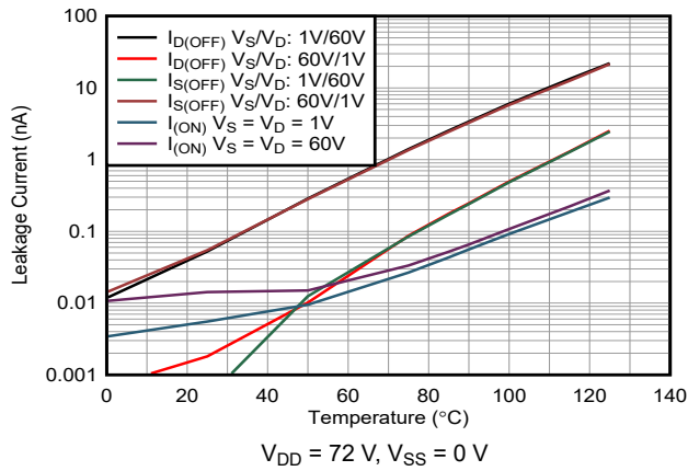
图 7-13. Leakage Current vs Temperature
