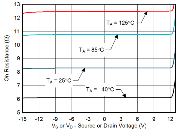
图 7-4. On-Resistance vs Source or Drain Voltage
