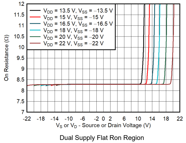
图 7-2. On-Resistance vs Source or Drain Voltage
