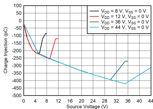
图 7-26. Charge Injection vs Source Voltage - Single Supply
