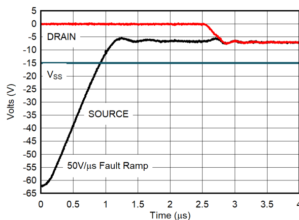
图 7-38. Drain Output Recovery - Negative Overvoltage
