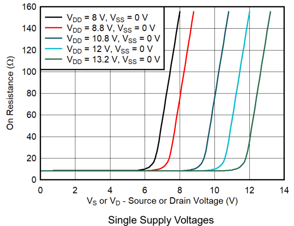
图 7-6. On-Resistance vs Source or Drain Voltage
