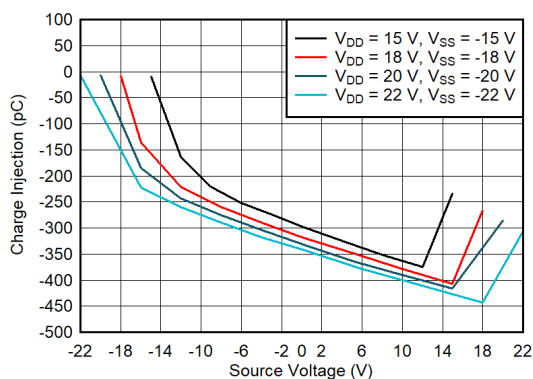
图 7-25. Charge Injection vs Source Voltage - Dual Supply
