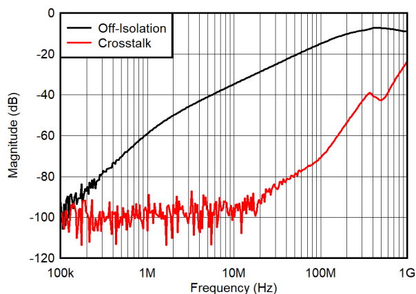
图 7-29. Crosstalk and Off Isolation vs Frequency
