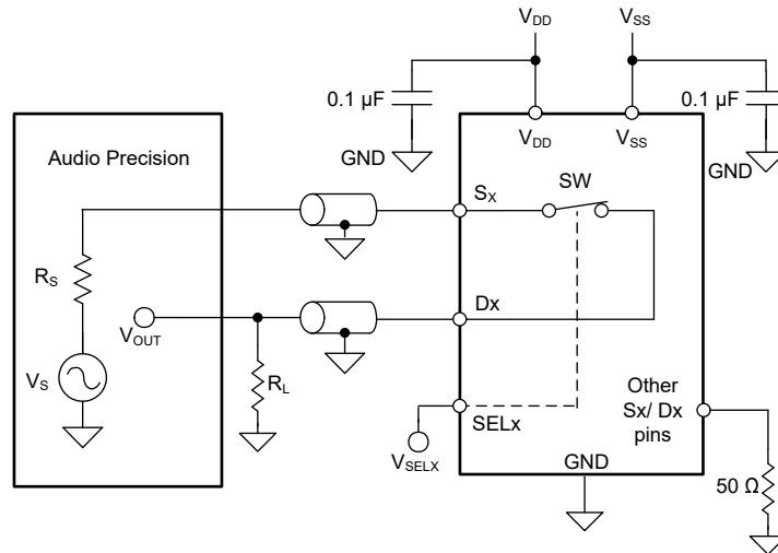
图 8-15. THD+N Measurement Setup
