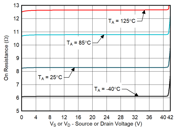
图 7-12. On-Resistance vs Source or Drain Voltage
