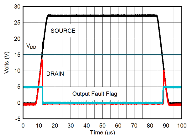
图 7-32. Fault Response and Recovery
