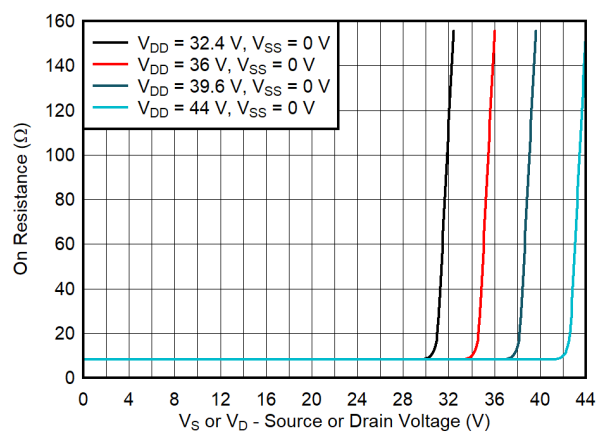
图 7-9. On-Resistance vs Source or Drain Voltage
