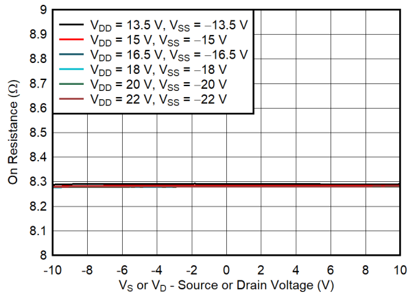
图 7-3. On-Resistance vs Source or Drain Voltage
