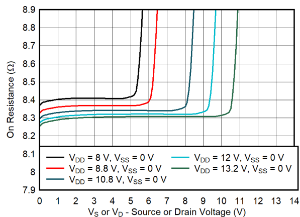
图 7-7. On-Resistance vs Source or Drain Voltage
