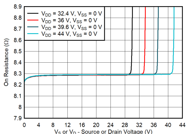
图 7-10. On-Resistance vs Source or Drain Voltage
