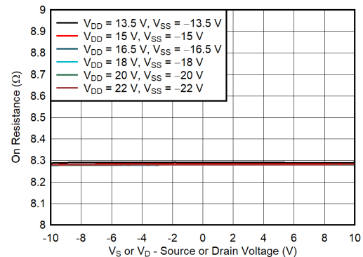
图 10-3. R_{ON} Flatness in Non-Fault Region
