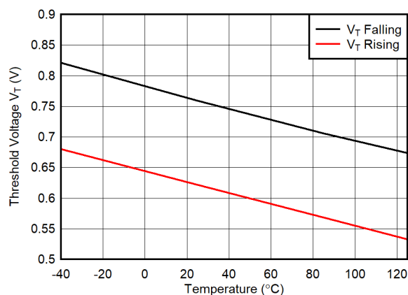
图 7-31. Threshold Voltage vs Temperature
