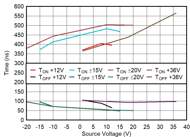
图 7-27. t_{ON} and t_{OFF} vs Source Voltage
