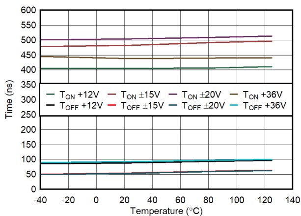
图 7-28. t_{ON} and t_{OFF} vs Temperature
