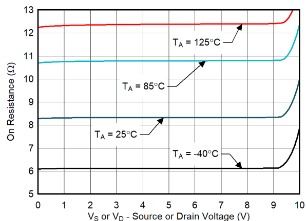
图 7-8. On-Resistance vs Source or Drain Voltage
