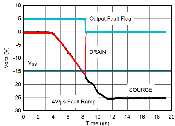
图 7-36. Drain Output Response - Negative Overvoltage
