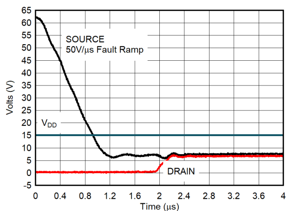
图 7-37. Drain Output Recovery - Positive Overvoltage
