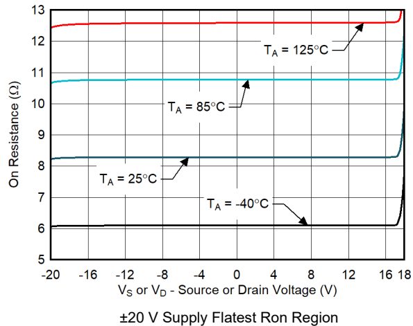
图 7-5. On-Resistance vs Source or Drain Voltage
