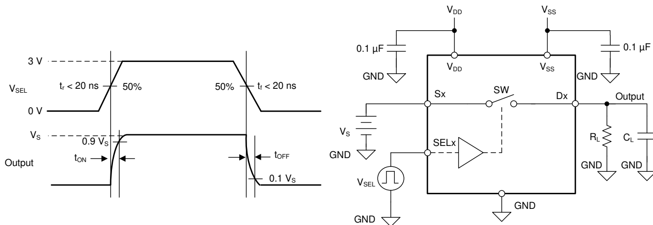
图 8-2. t_{ON} and t_{OFF} Measurement Setup
