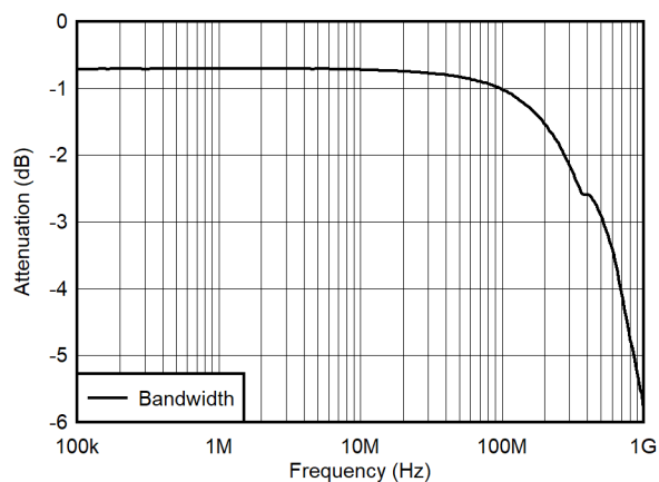
图 7-30. Insertion Loss vs Frequency
