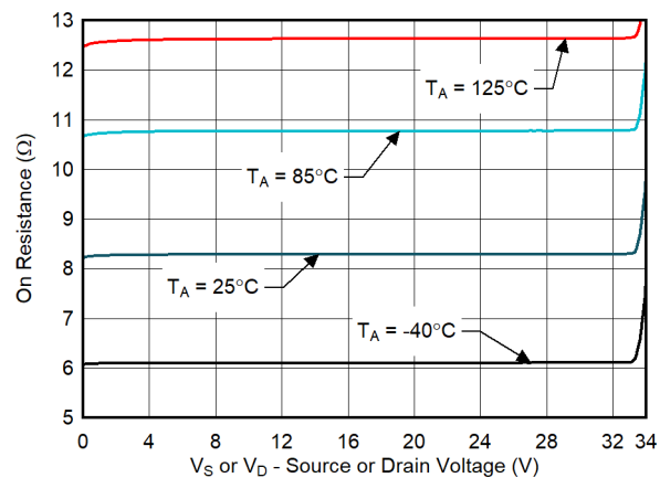
图 7-11. On-Resistance vs Source or Drain Voltage
