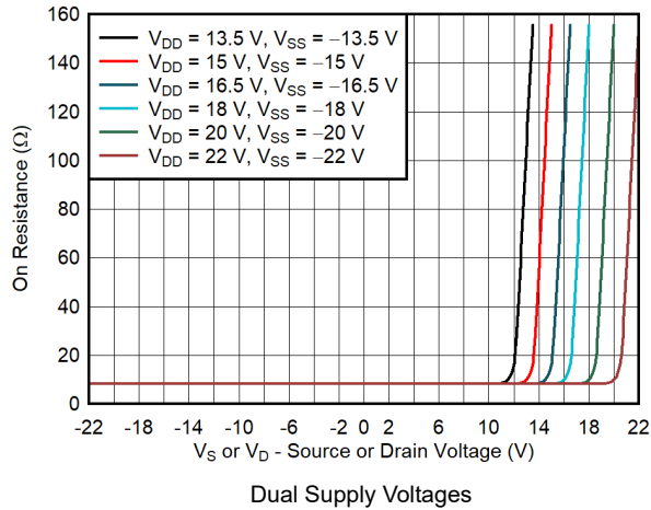
图 7-1. On-Resistance vs Source or Drain Voltage
