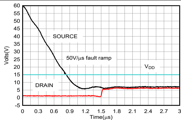
图 7-37. Drain Output Response - Positive Overvoltage
