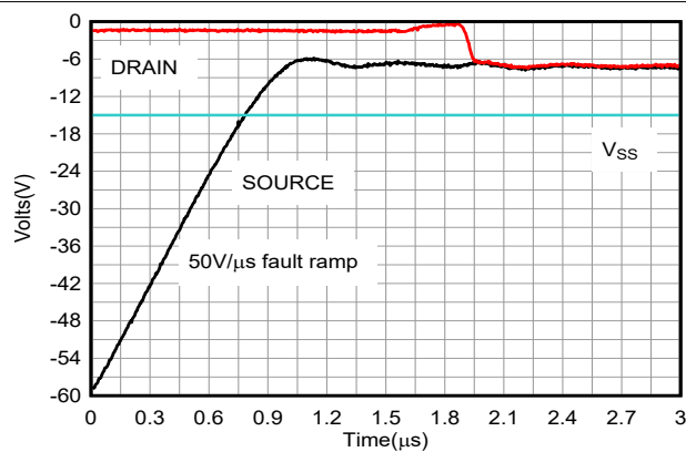
图 7-38. Drain Output Response - Negative Overvoltage
