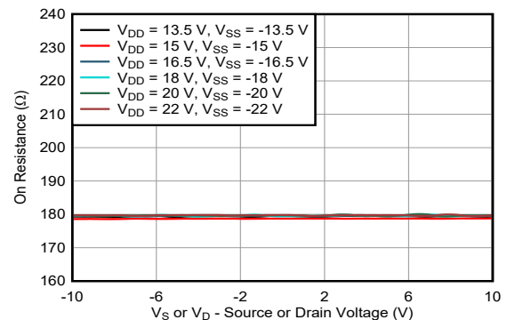
图 10-3. R_{ON} Flatness in Non-Fault Region
