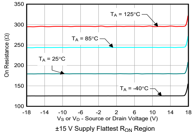
图 7-4. On-Resistance vs Source or Drain Voltage
