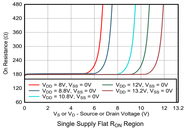
图 7-7. On-Resistance vs Source or Drain Voltage
