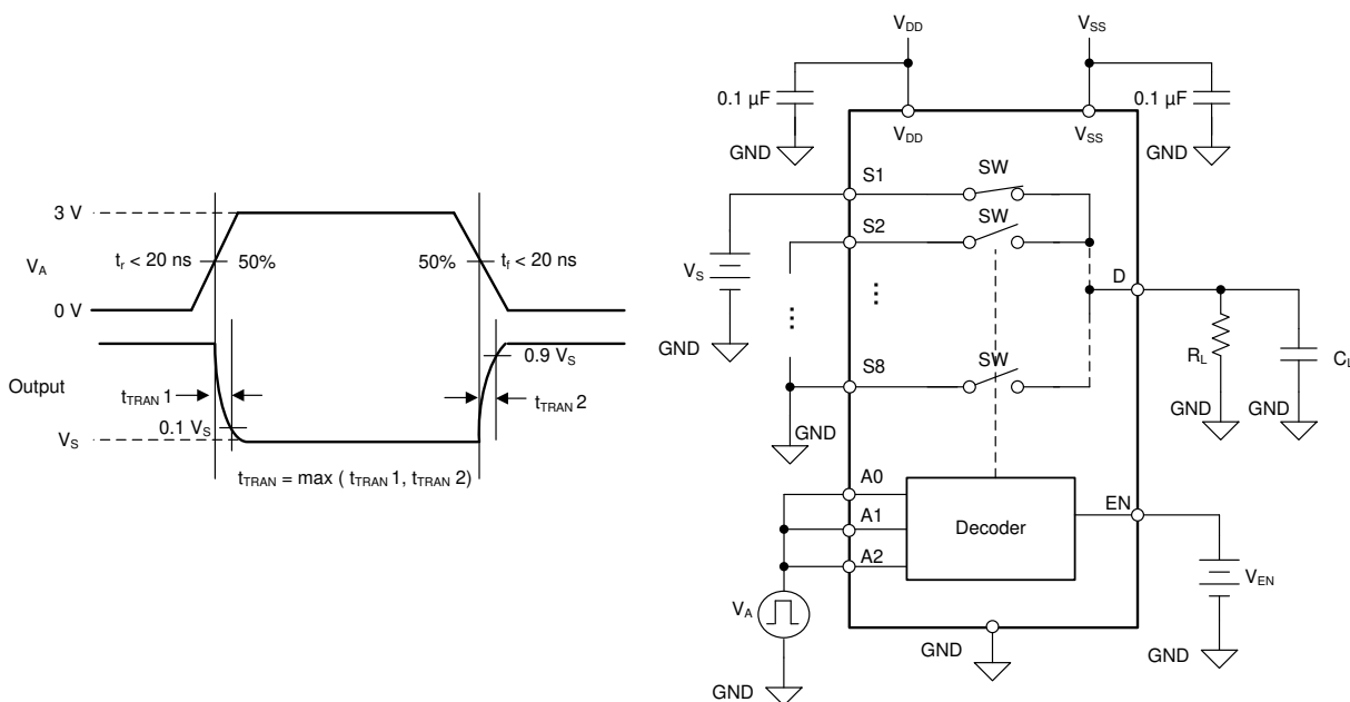
图 8-8. Transition Time Measurement Setup
