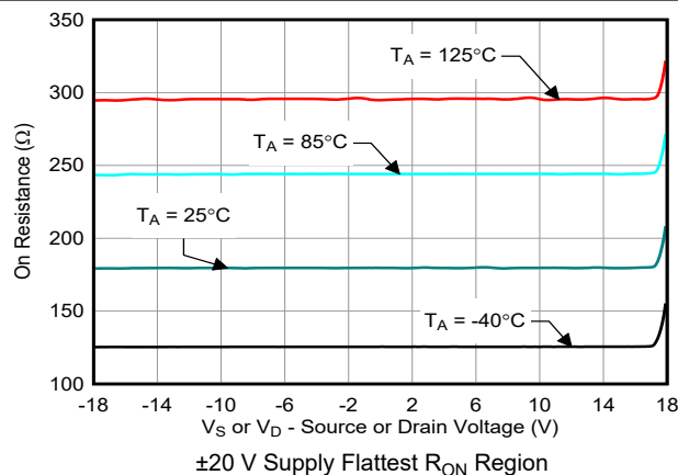
图 7-5. On-Resistance vs Source or Drain Voltage
