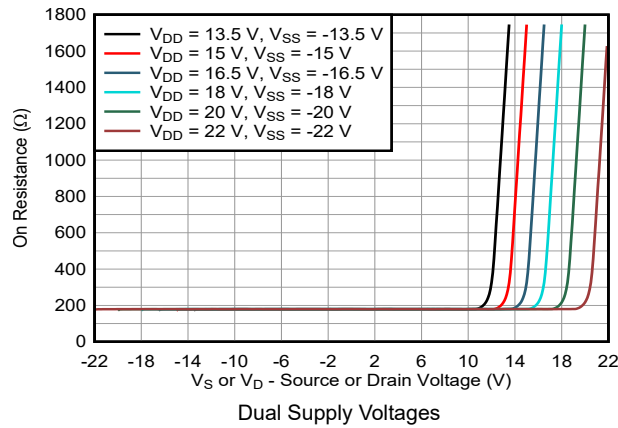
图 7-1. On-Resistance vs Source or Drain Voltage
