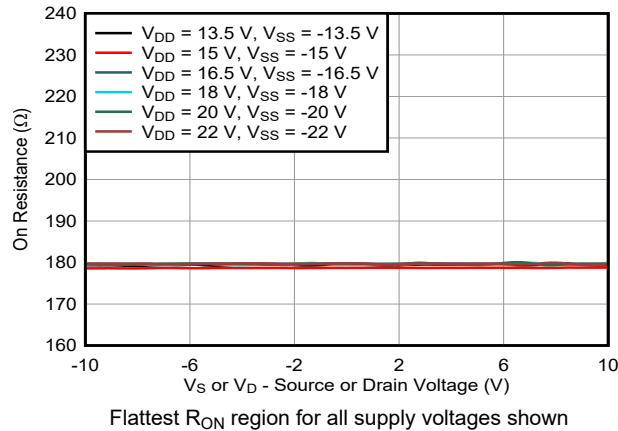
图 7-3. On-Resistance vs Source or Drain Voltage
