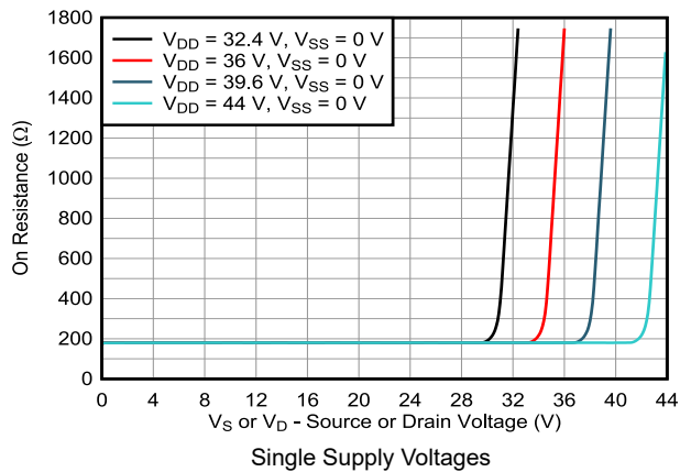
图 7-9. On-Resistance vs Source or Drain Voltage
