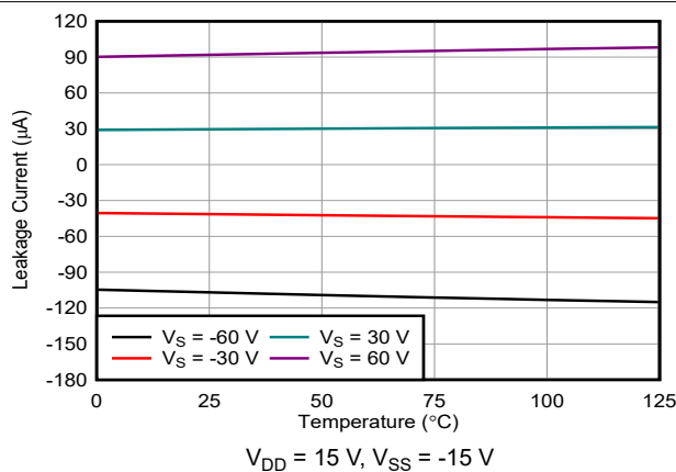
图 7-23. I_{S(FA)} Overvoltage Leakage Current vs Temperature
