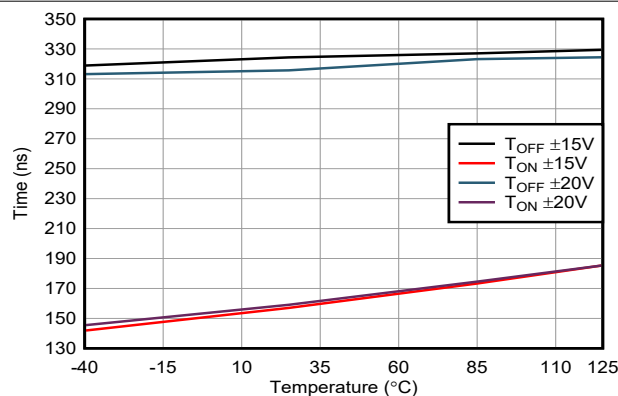
图 7-27. Transition Times vs Temperature
