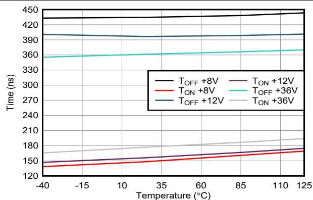
图 7-28. Transition Times vs Temperature
