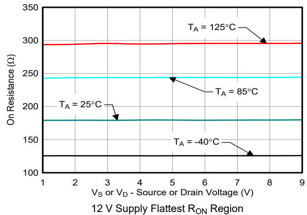
图 7-8. On-Resistance vs Source or Drain Voltage
