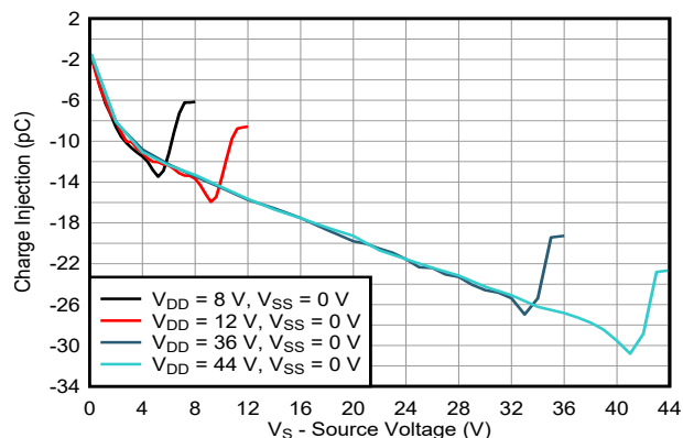
图 7-26. Charge Injection vs Source Voltage - Single Supply
