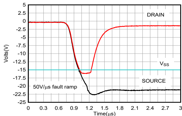
图 7-38. Drain Output Response - Negative Overvoltage
