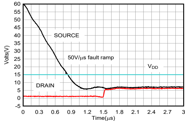
图 7-37. Drain Output Response - Positive Overvoltage
