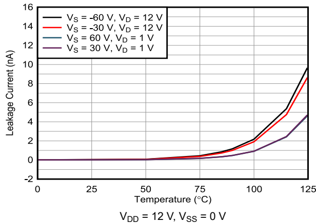
图 7-21. I_{D(FA)} Overvoltage Leakage Current vs Temperature
