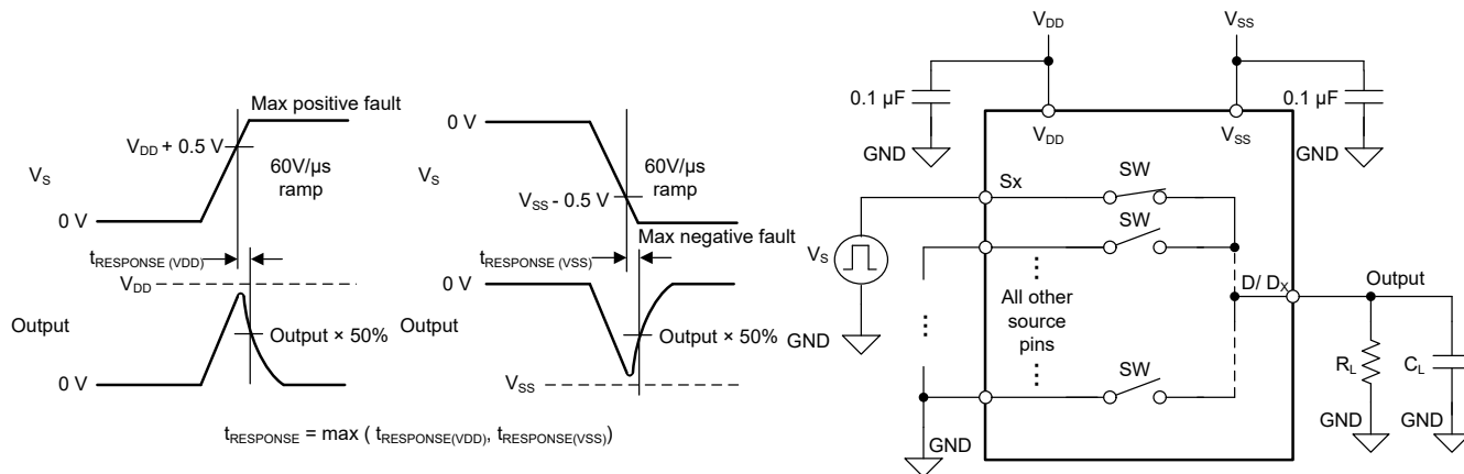
图 8-9. Fault Response Time Measurement Setup
