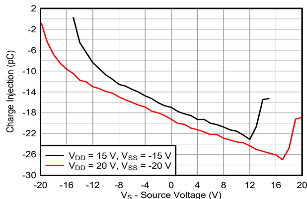
图 7-25. Charge Injection vs Source Voltage - Dual Supply
