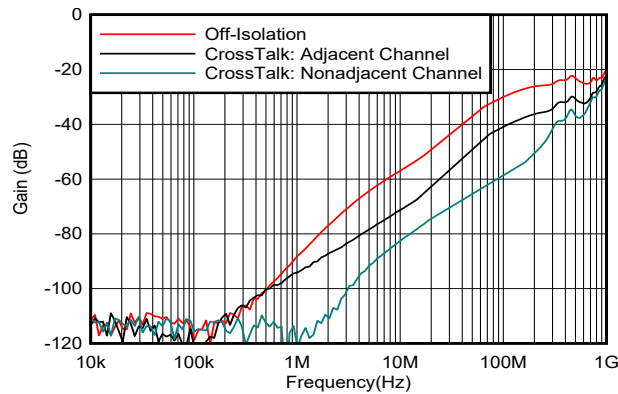
图 7-31. Off Isolation and Crosstalk vs Frequency
