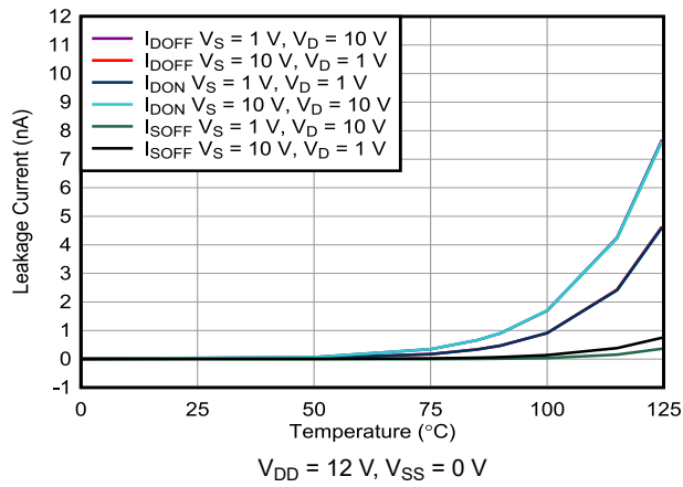
图 7-13. Leakage Current vs Temperature
