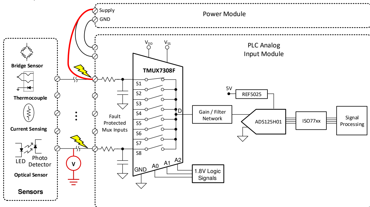
图 10-1. Typical Application
