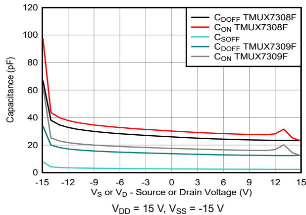
图 7-33. Capacitance vs Source or Drain Voltage
