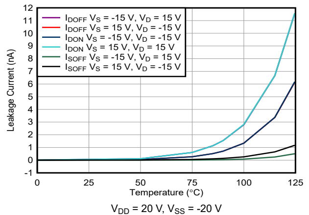
图 7-16. Leakage Current vs Temperature
