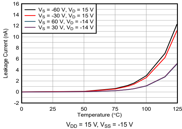
图 7-19. I_{D(FA)} Overvoltage Leakage Current vs Temperature
