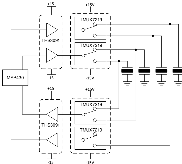
图 8-3. Ultrasonic Sensing Gas Meter System
