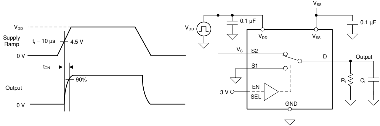
图 6-7. t_{ON(VDD)} Time Measurement Setup
