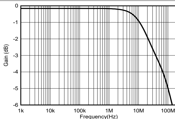
图 5-24. On Response vs Frequency
