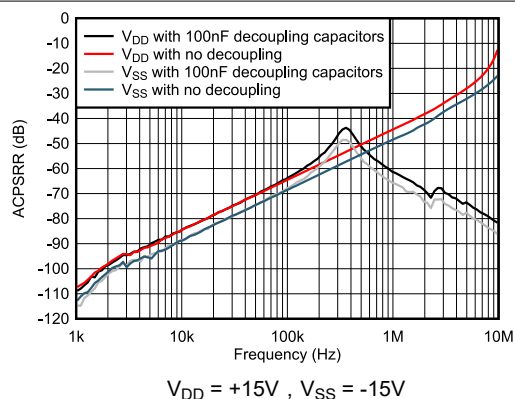
图 5-29. ACPSR vs Frequency
