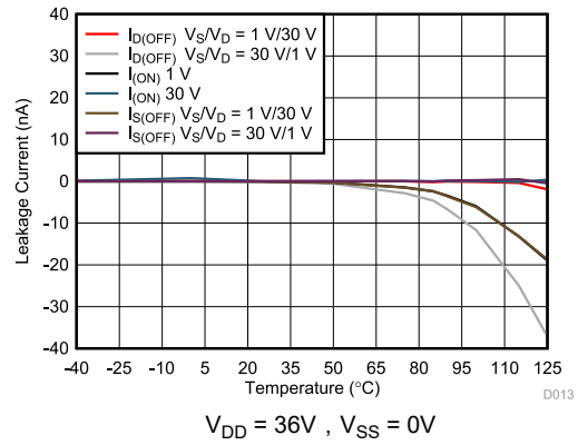
图 5-12. Leakage Current vs Temperature
