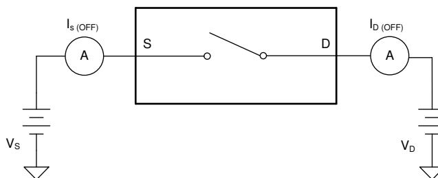
图 8-2. Off-Leakage Measurement Setup
